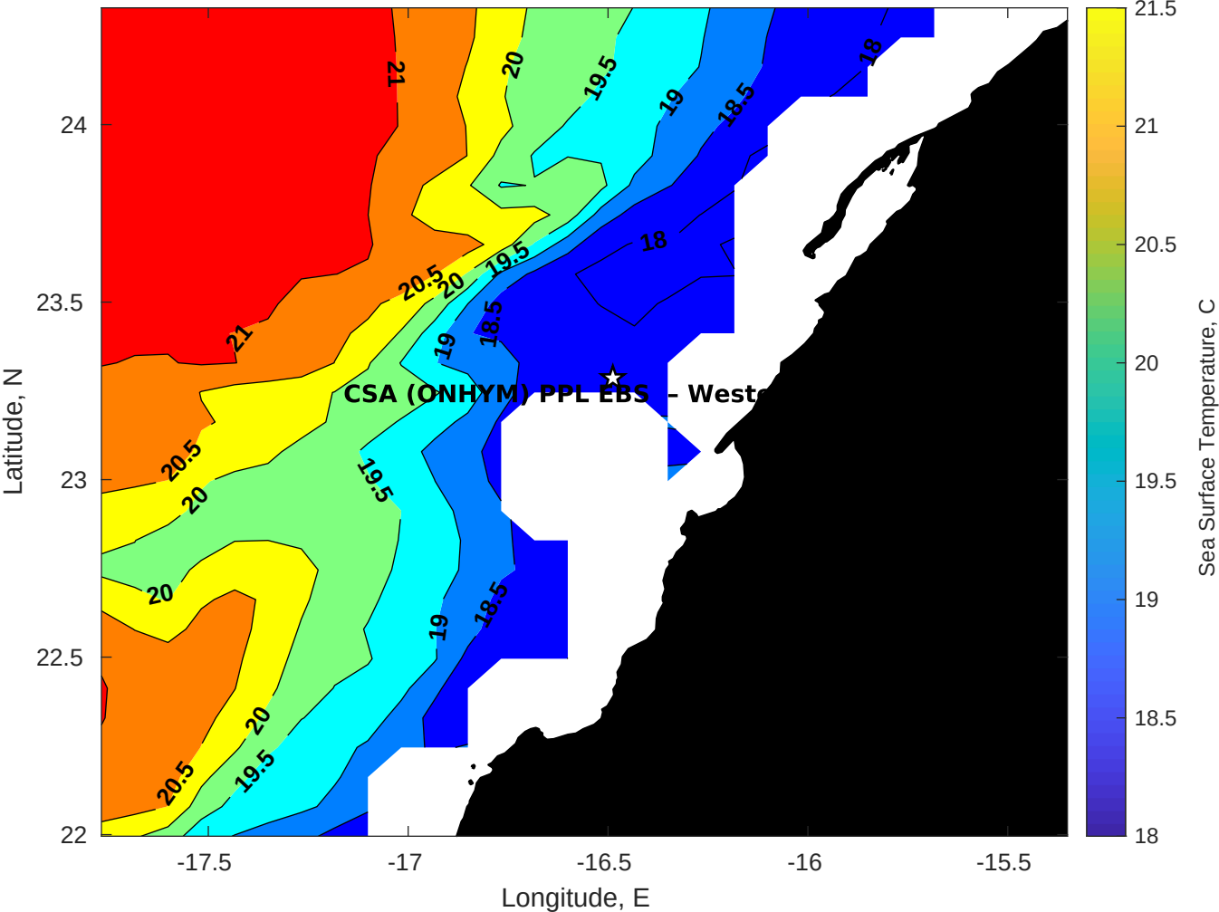
SST for CSA (ONHYM) PPL EBS - Western Sahara at 18-May-2025 00:00:00
