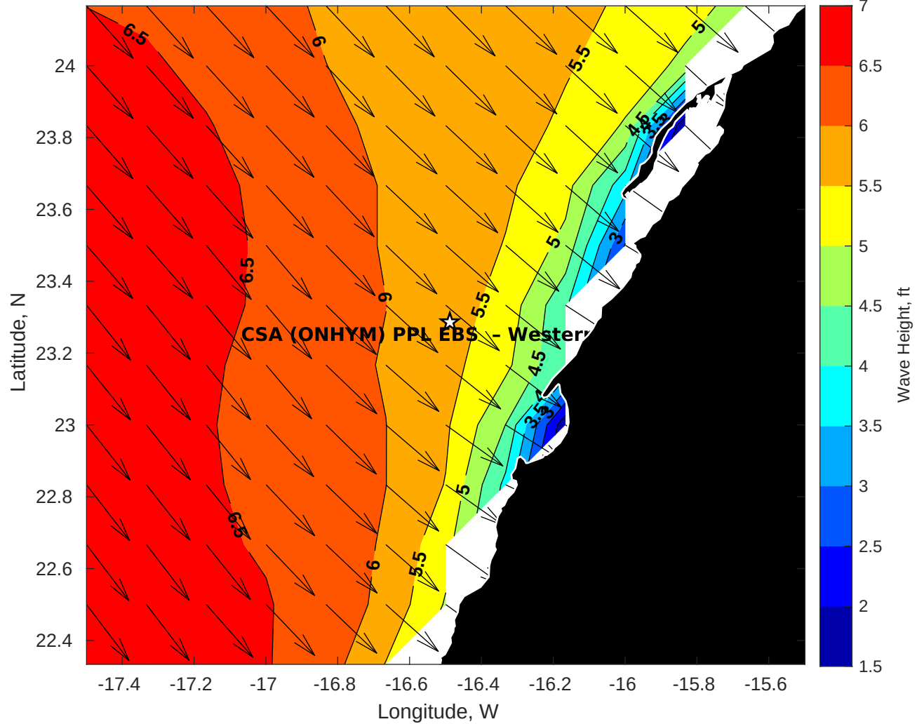
Wave Height (ft) for CSA (ONHYM) PPL EBS - Western Sahara at 19-May-2025 09:00:00
