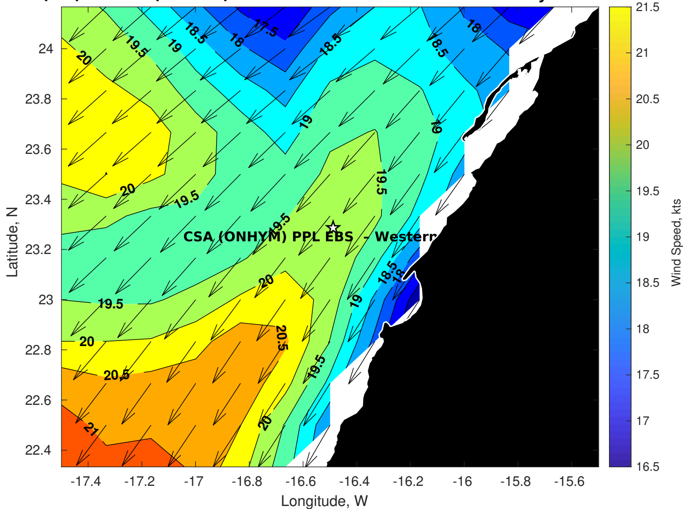
Winds (kts) for CSA (ONHYM) PPL EBS - Western Sahara at 19-May-2025 09:00:00
