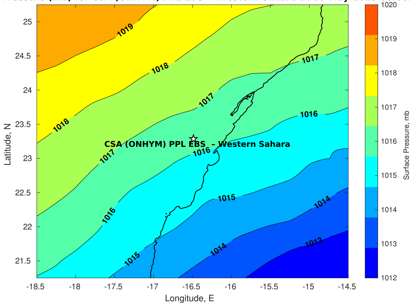
Surface Pressure (mb) for CSA (ONHYM) PPL EBS - Western Sahara at 20-May-2025 00:00:00
