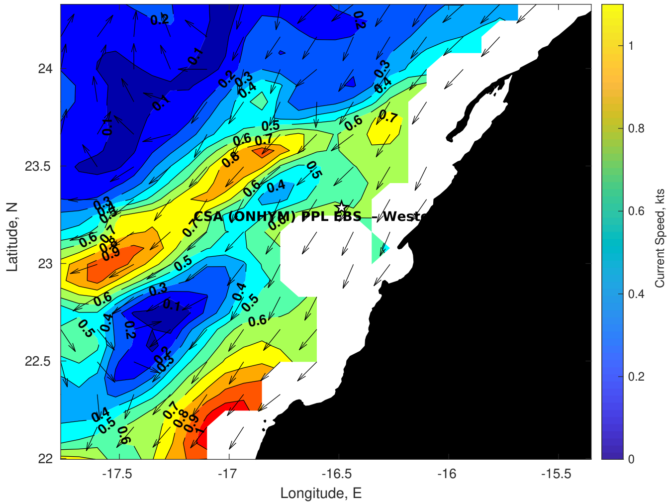
Surface Currents for CSA (ONHYM) PPL EBS - Western Sahara at 18-May-2025 00:00:00
