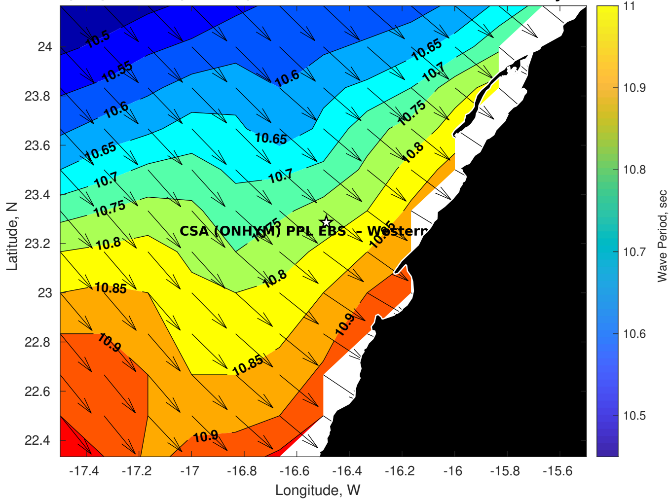
Wave Period (sec) for CSA (ONHYM) PPL EBS - Western Sahara at 19-May-2025 09:00:00
