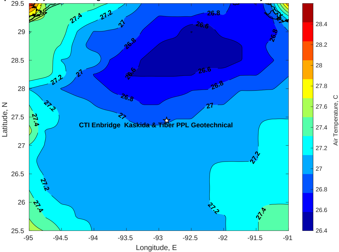
Air Temperature (C) for CTI Enbridge Kaskida & Tiber PPL Geotechnical at 19-May-2025
