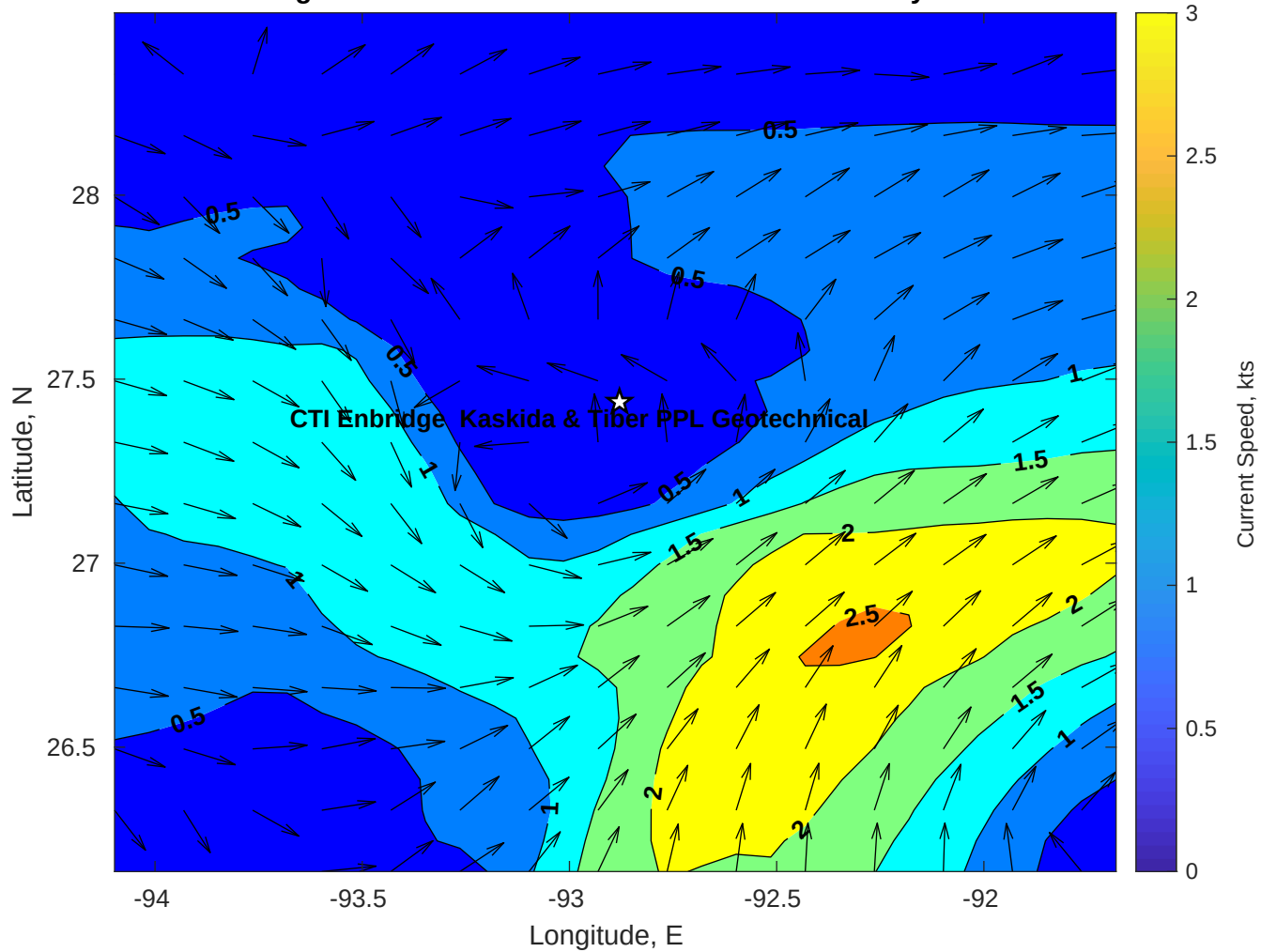
Surface Currents for CTI Enbridge Kaskida & Tiber PPL Geotechnical at 18-May-2025 00:00:00
