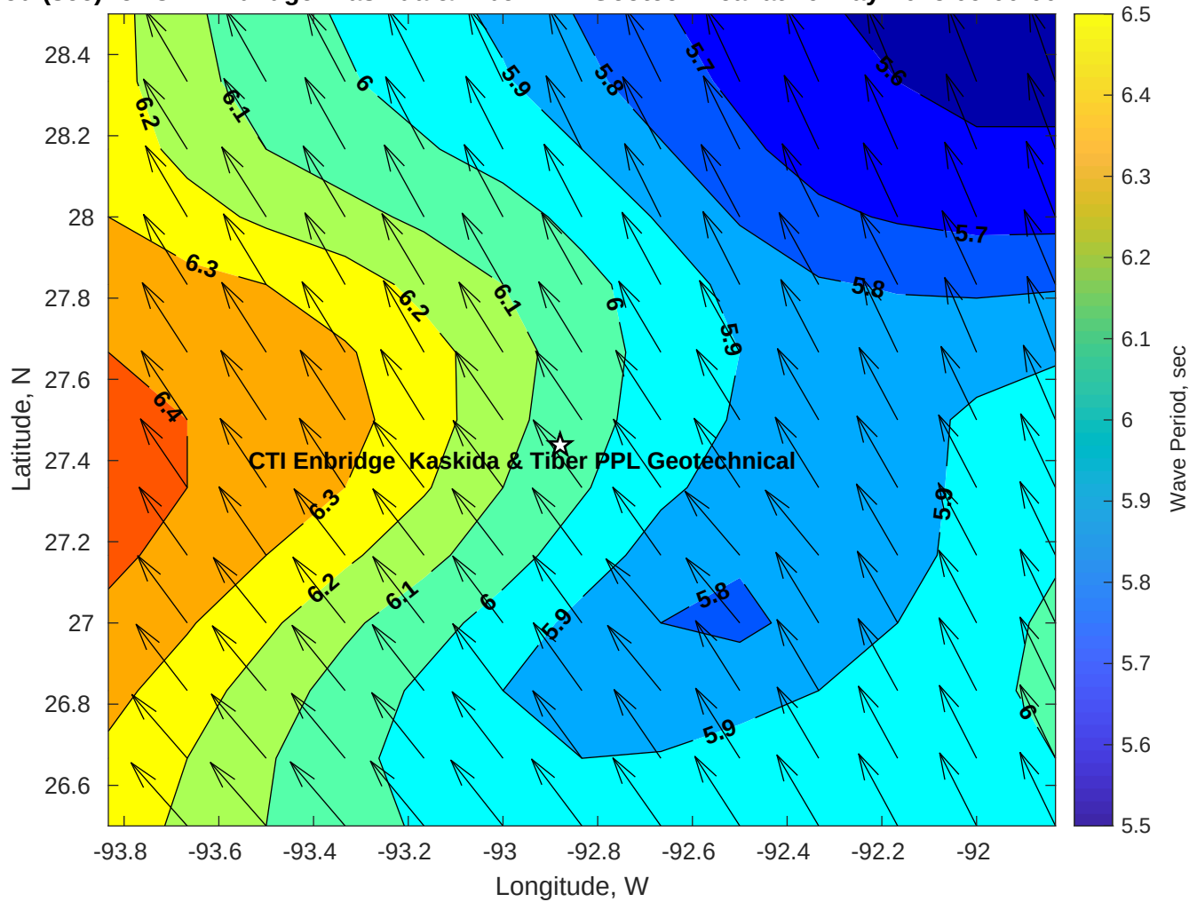
Wave Period (sec) for CTI Enbridge Kaskida & Tiber PPL Geotechnical at 19-May-2025 09:00:00
