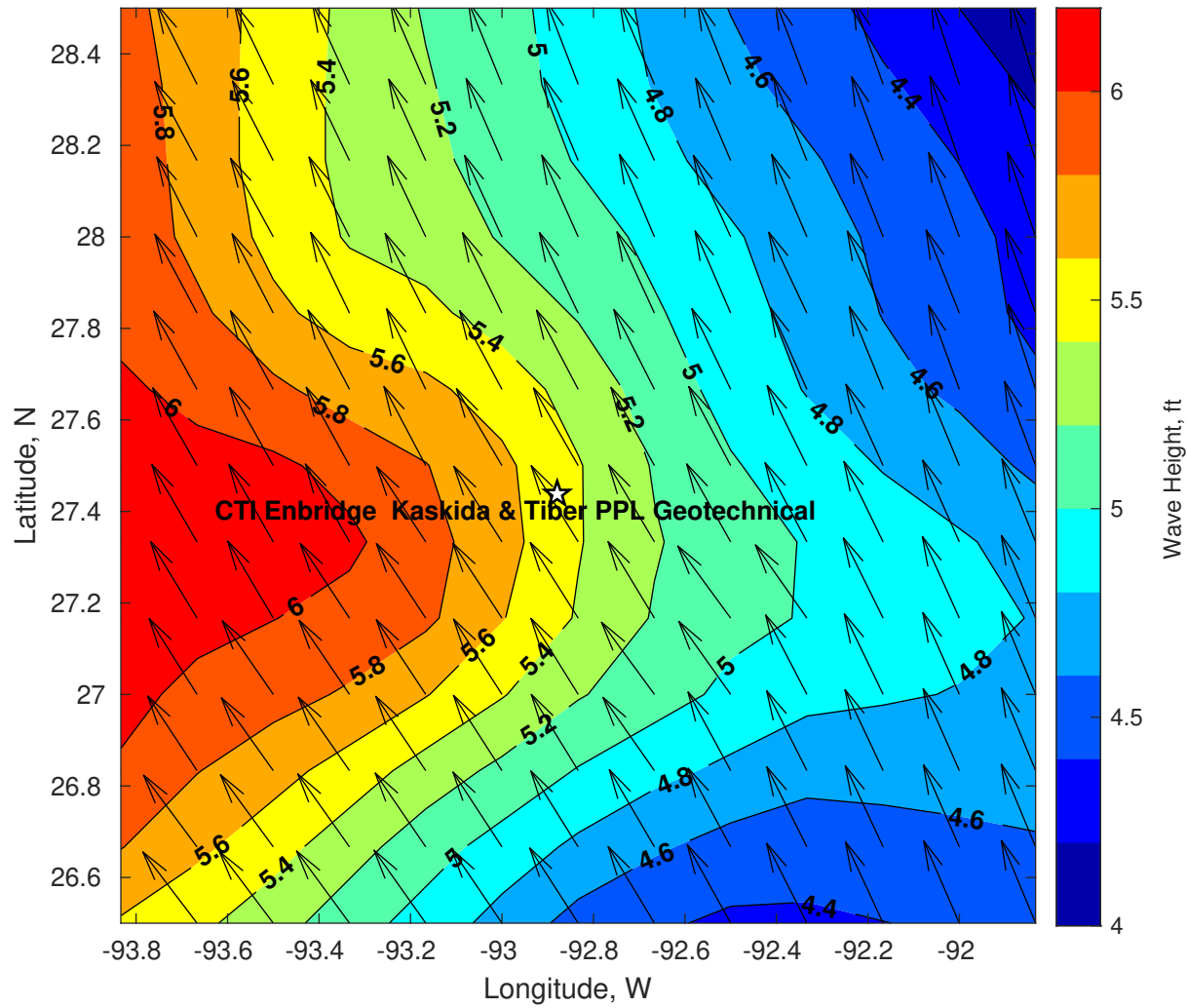
Wave Height (ft) for CTI Enbridge Kaskida & Tiber PPL Geotechnical at 19-May-2025 09:00:00
