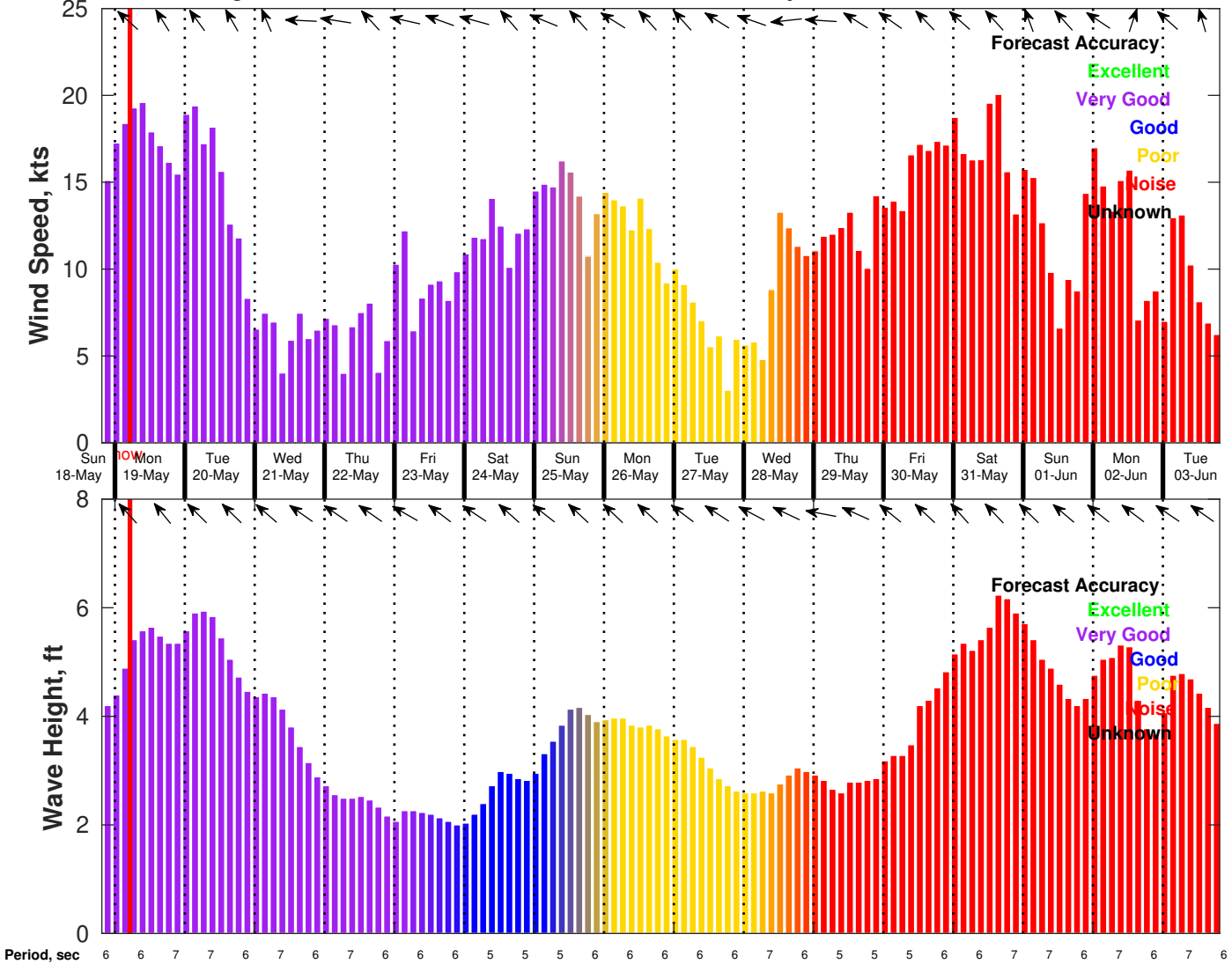
Wind & Wave Forecast for CTI Enbridge Kaskida & Tiber PPL Geotechnical from 18-May-2025 20:00:00 to 03-Jun-2025 20:00:00
