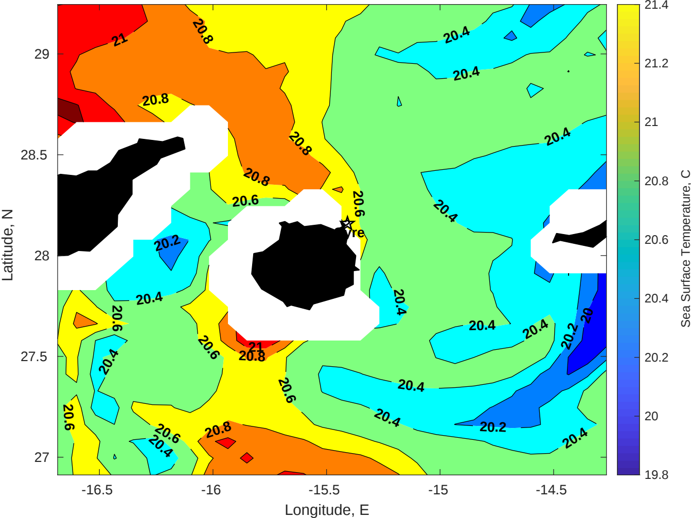
SST for Gyre at 18-May-2025 00:00:00
