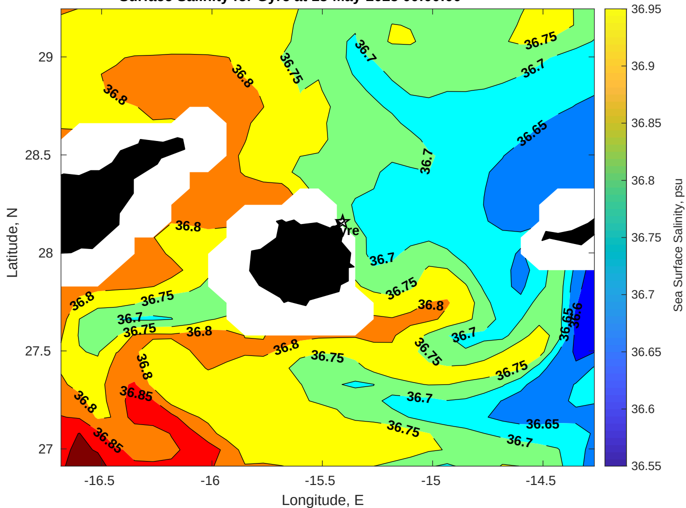
Surface Salinity for Gyre at 18-May-2025 00:00:00
