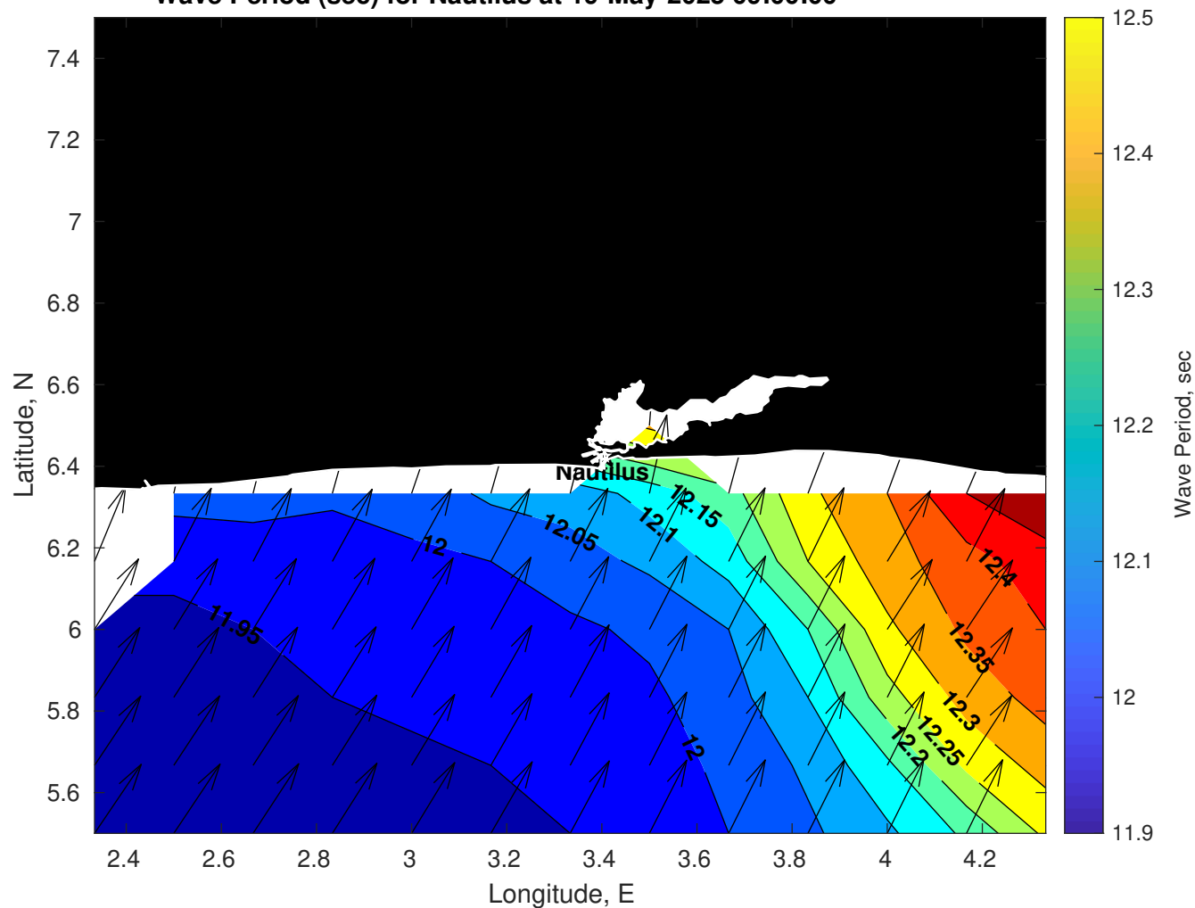
Wave Period (sec) for Nautilus at 19-May-2025 09:00:00
