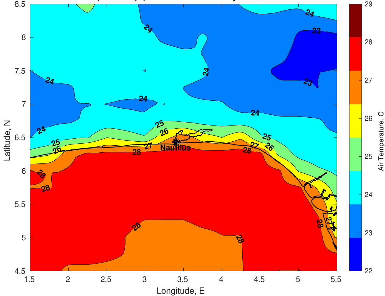
Air Temperature (C) for Nautilus at 19-May-2025
