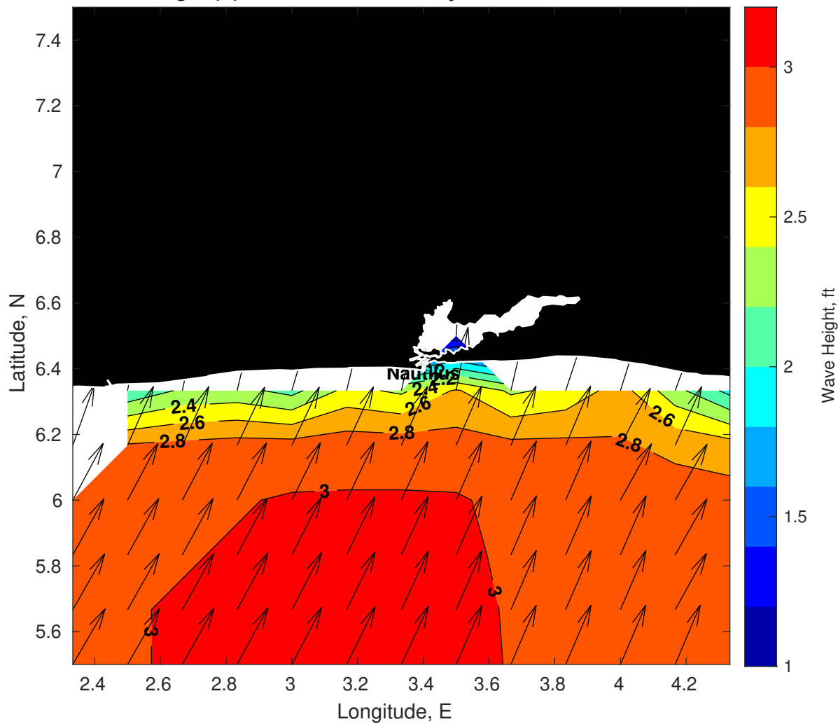
Wave Height (ft) for Nautilus at 19-May-2025 09:00:00
