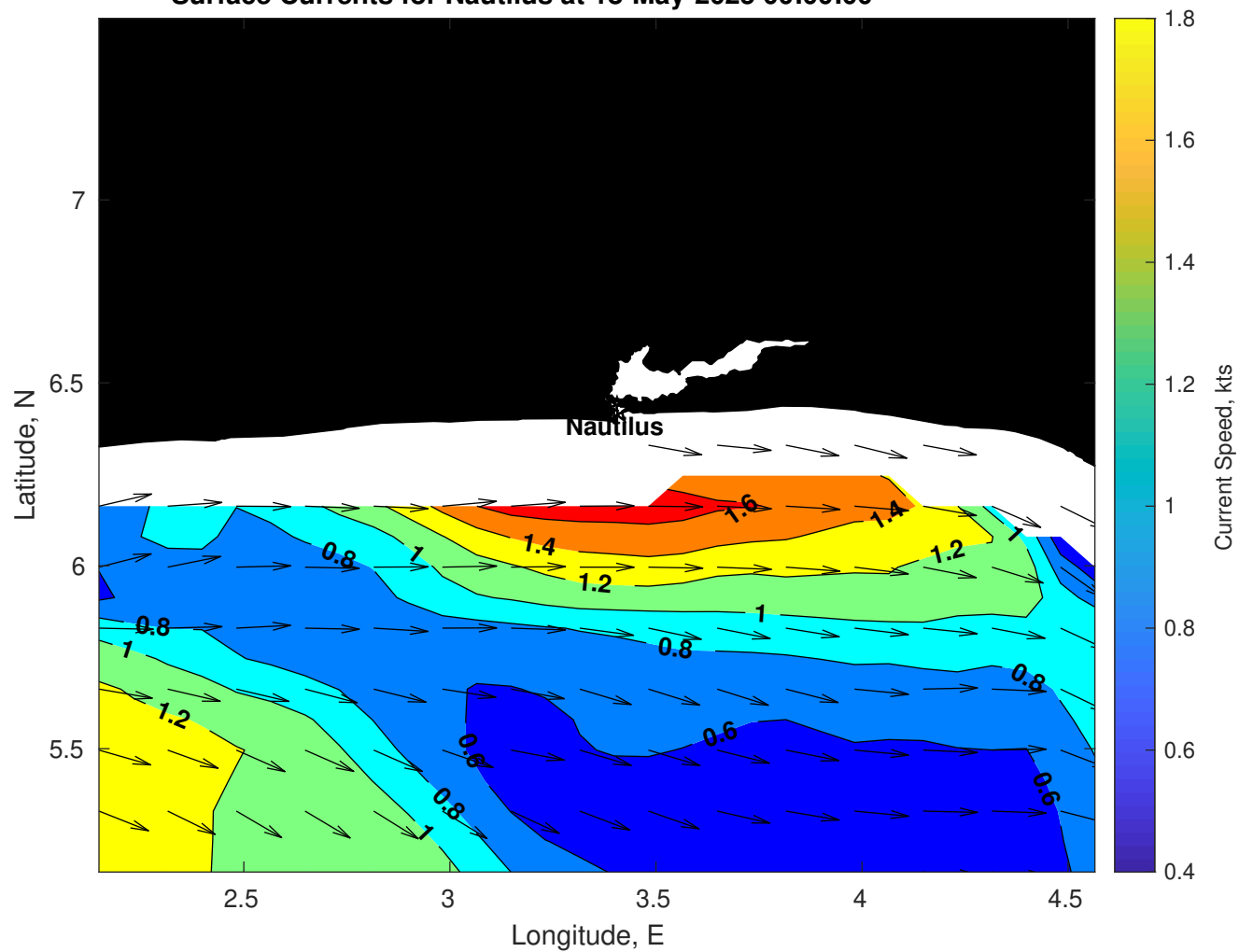
Surface Currents for Nautilus at 18-May-2025 00:00:00
