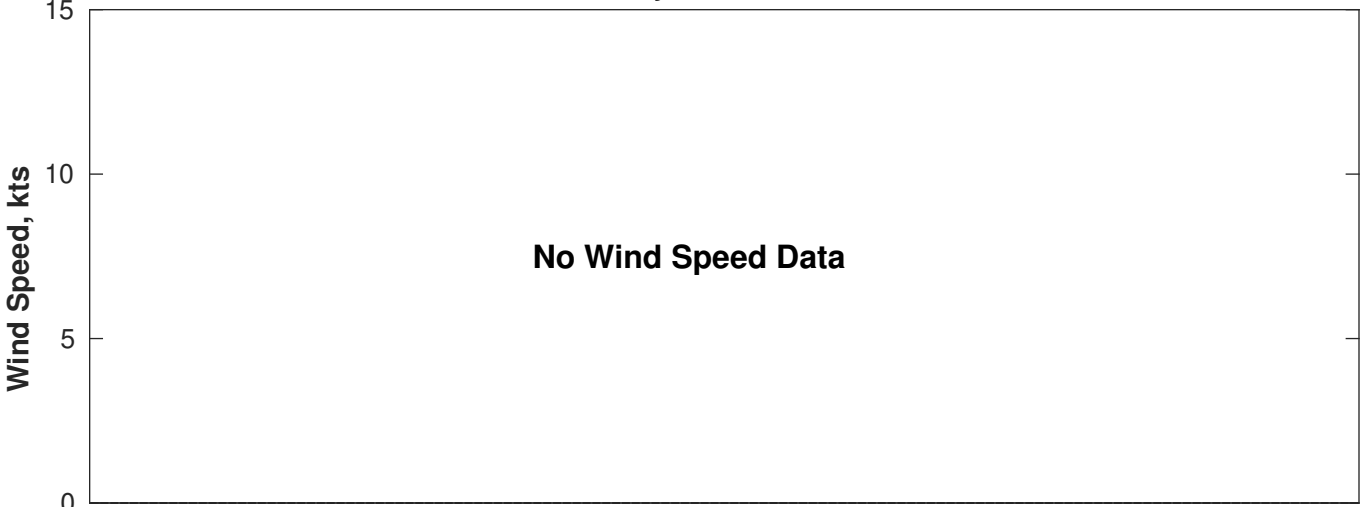
Wind & Wave Forecast for Nautilus from 19-May-2025 02:00:00 to 04-Jun-2025 02:00:00
