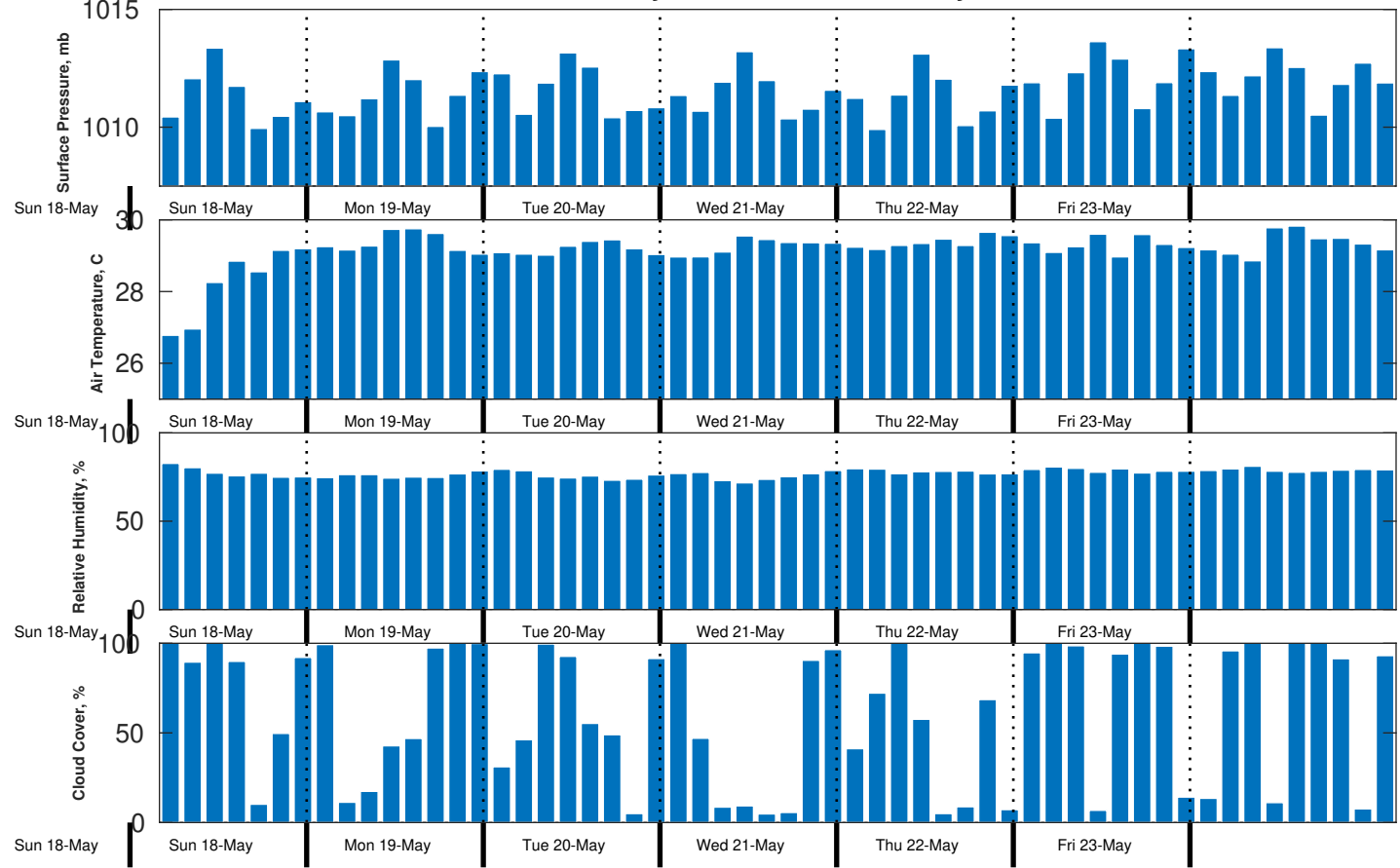
Met Forecast for Nautilus from 19-May-2025 00:00:00 to 26-May-2025 00:00:00
