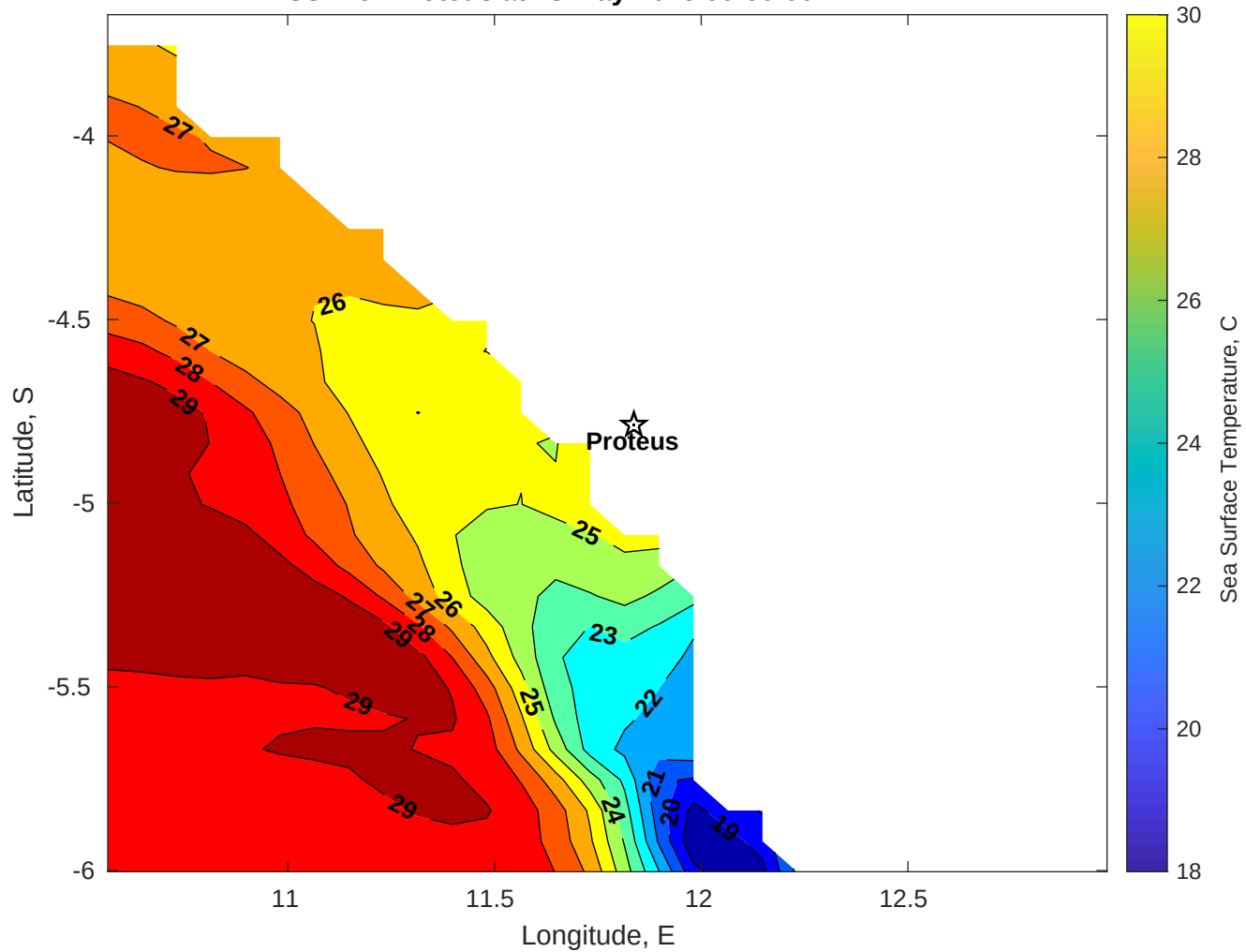
SST for Proteus at 18-May-2025 00:00:00
