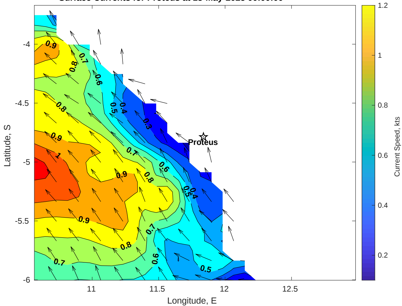
Surface Currents for Proteus at 18-May-2025 00:00:00
