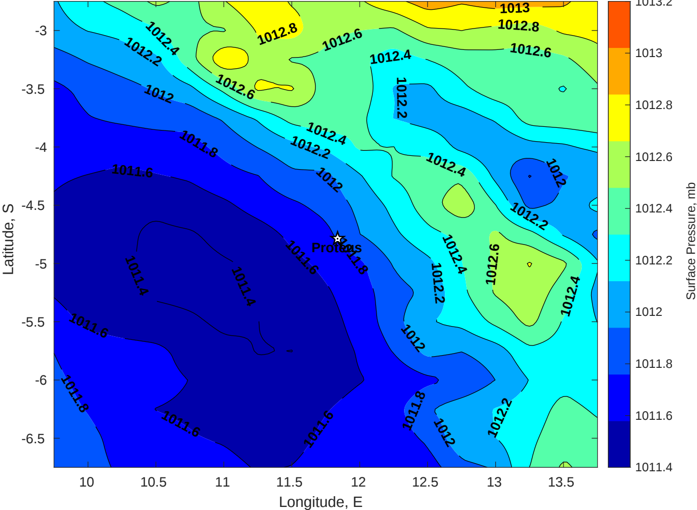
Surface Pressure (mb) for Proteus at 20-May-2025 00:00:00
