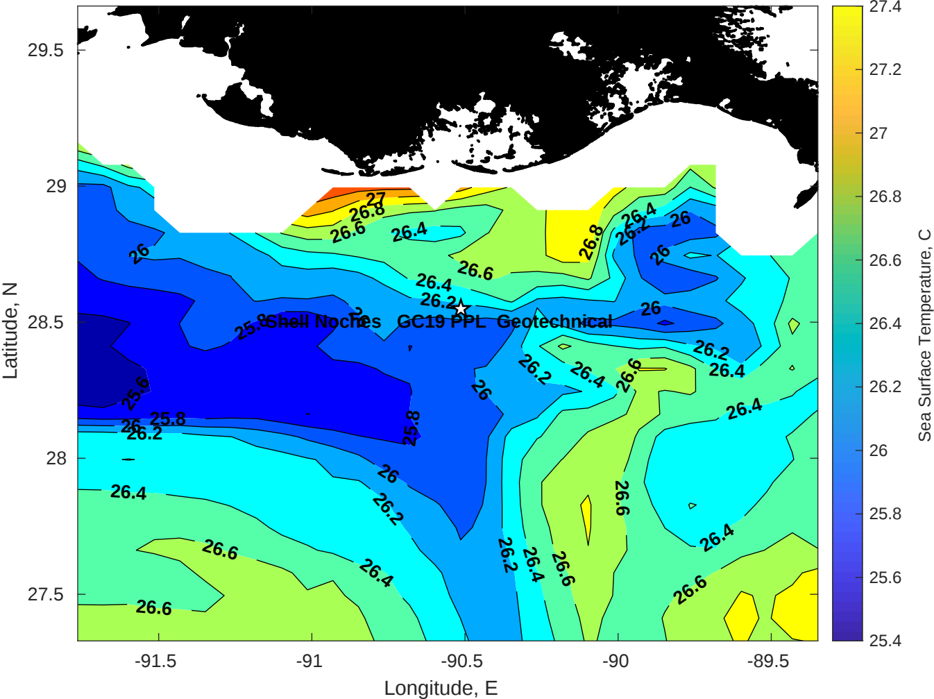
SST for Shell Noches GC19 PPL Geotechnical at 18-May-2025 00:00:00
