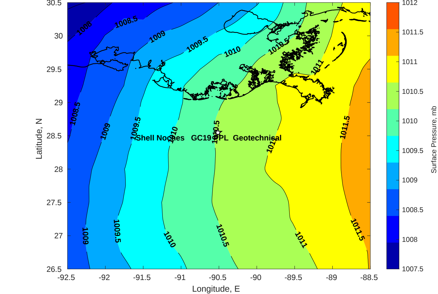
Surface Pressure (mb) for Shell Noches GC19 PPL Geotechnical at 20-May-2025 00:00:00
