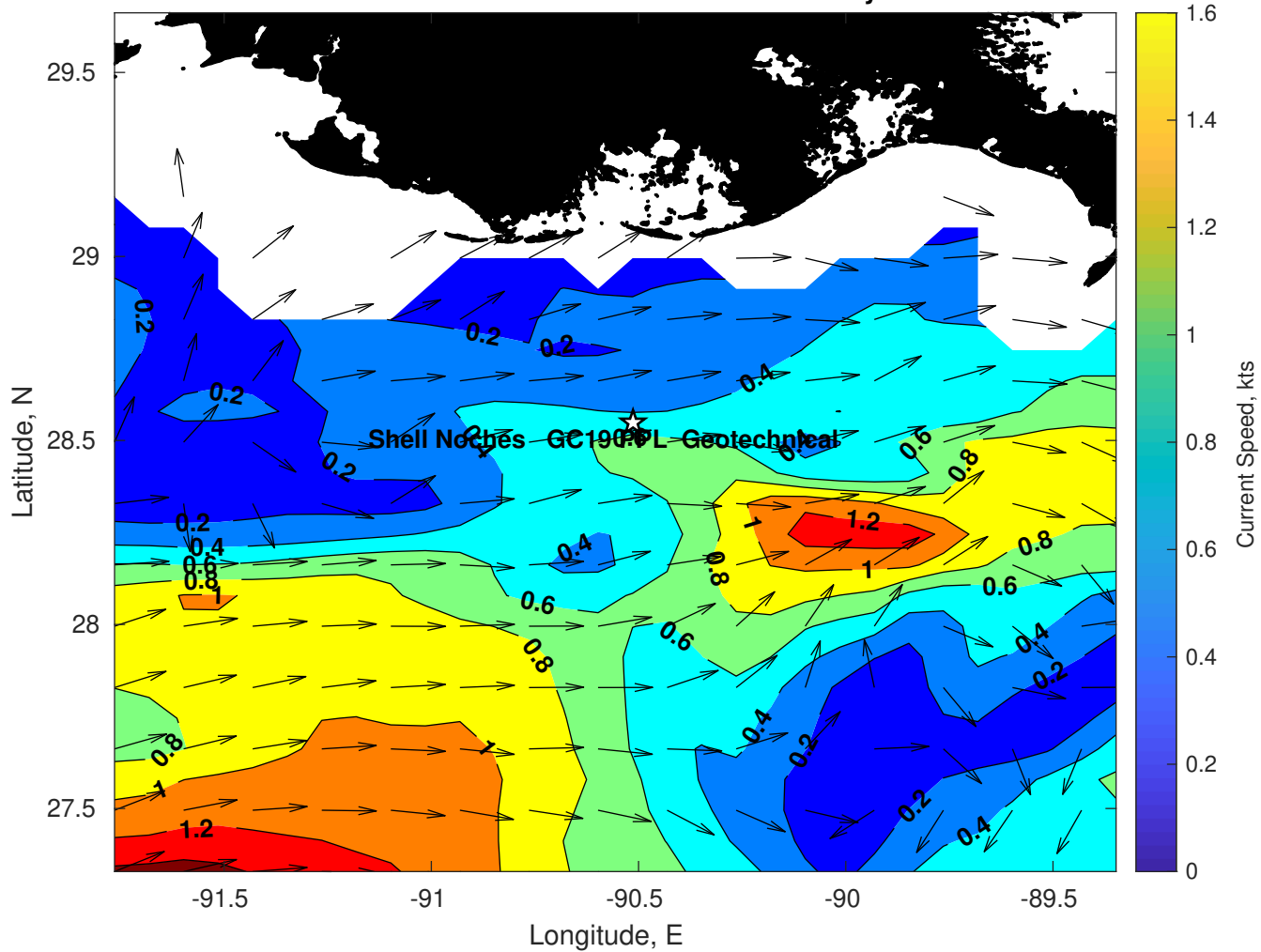
Surface Currents for Shell Noches GC19 PPL Geotechnical at 18-May-2025 00:00:00
