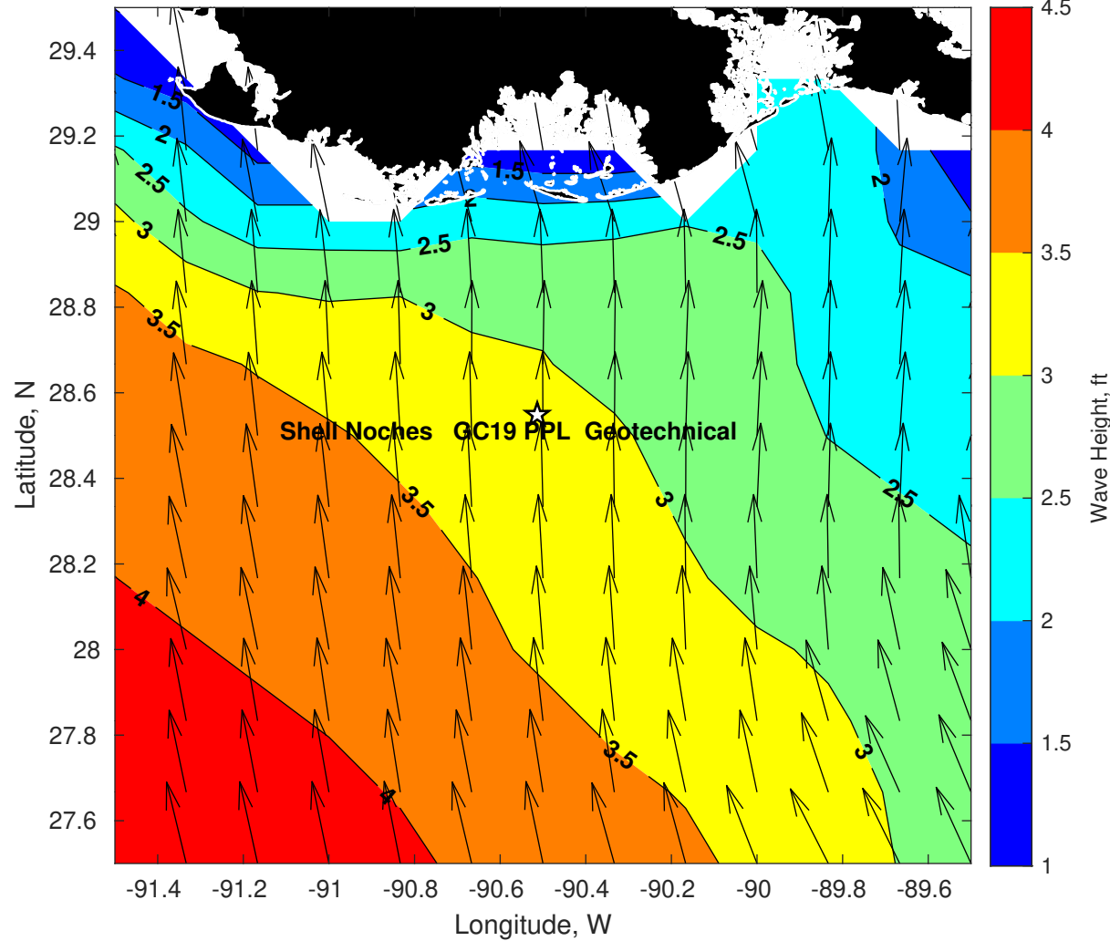
Wave Height (ft) for Shell Noches GC19 PPL Geotechnical at 19-May-2025 09:00:00
