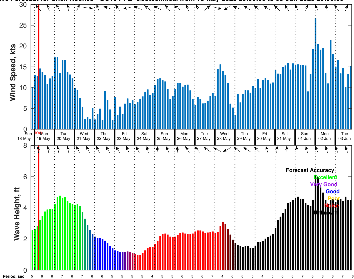
Wind & Wave Forecast for Shell Noches GC19 PPL Geotechnical from 18-May-2025 20:00:00 to 03-Jun-2025 20:00:00
