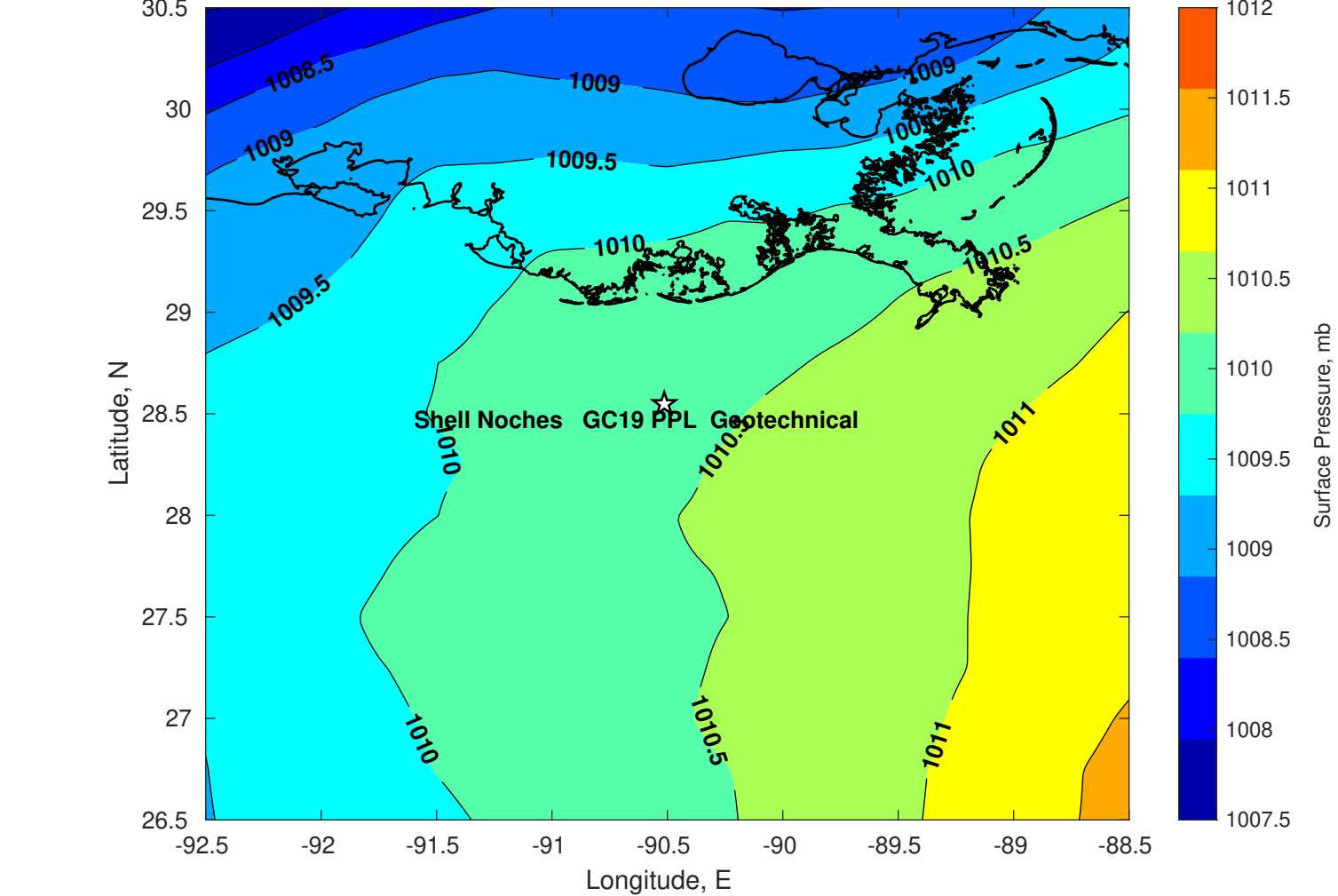
Surface Pressure (mb) for Shell Noches GC19 PPL Geotechnical at 21-May-2025 00:00:00
