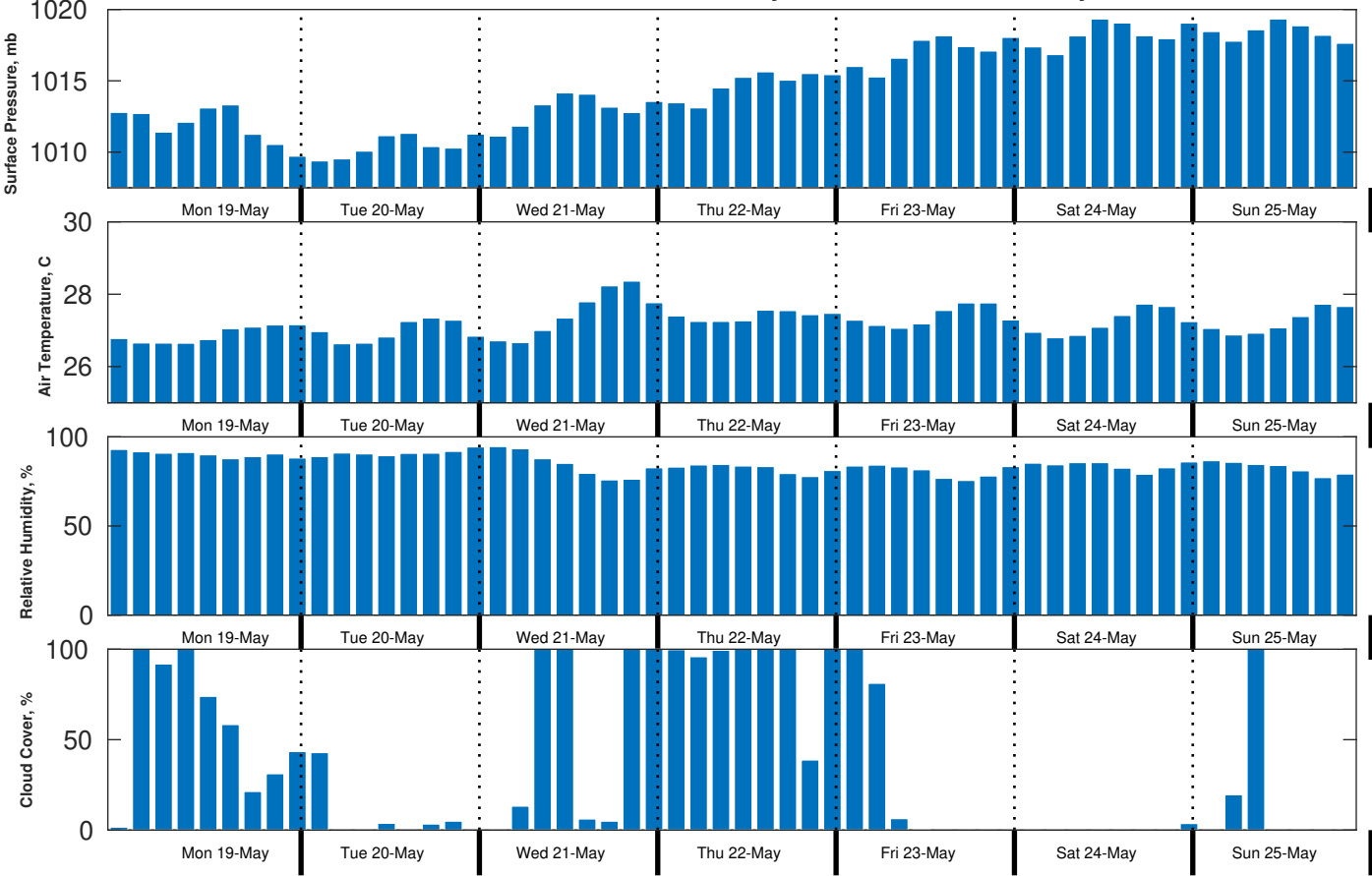
Met Forecast for Shell Noches GC19 PPL Geotechnical from 19-May-2025 00:00:00 to 26-May-2025 00:00:00
