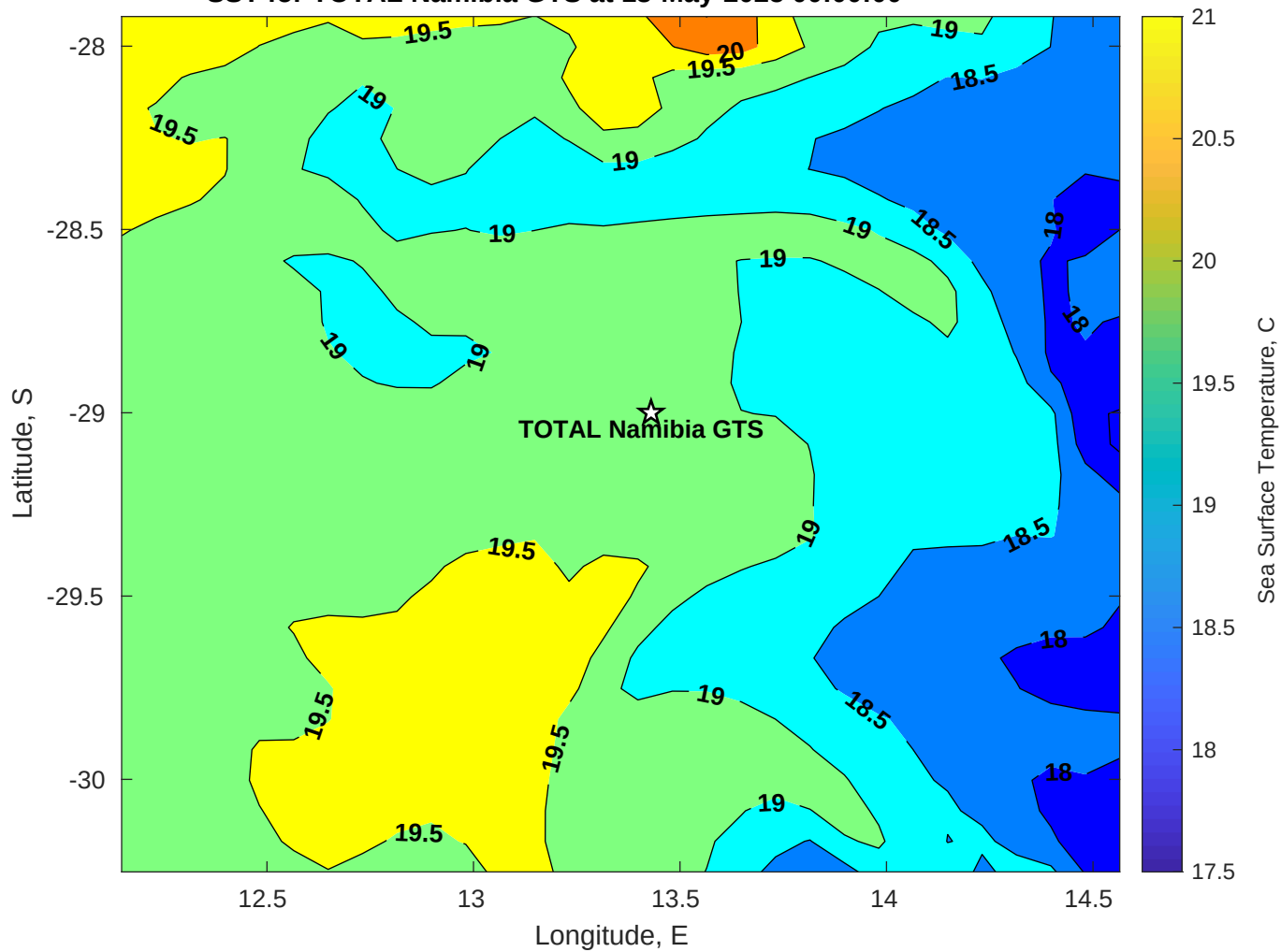
SST for TOTAL Namibia GTS at 18-May-2025 00:00:00
