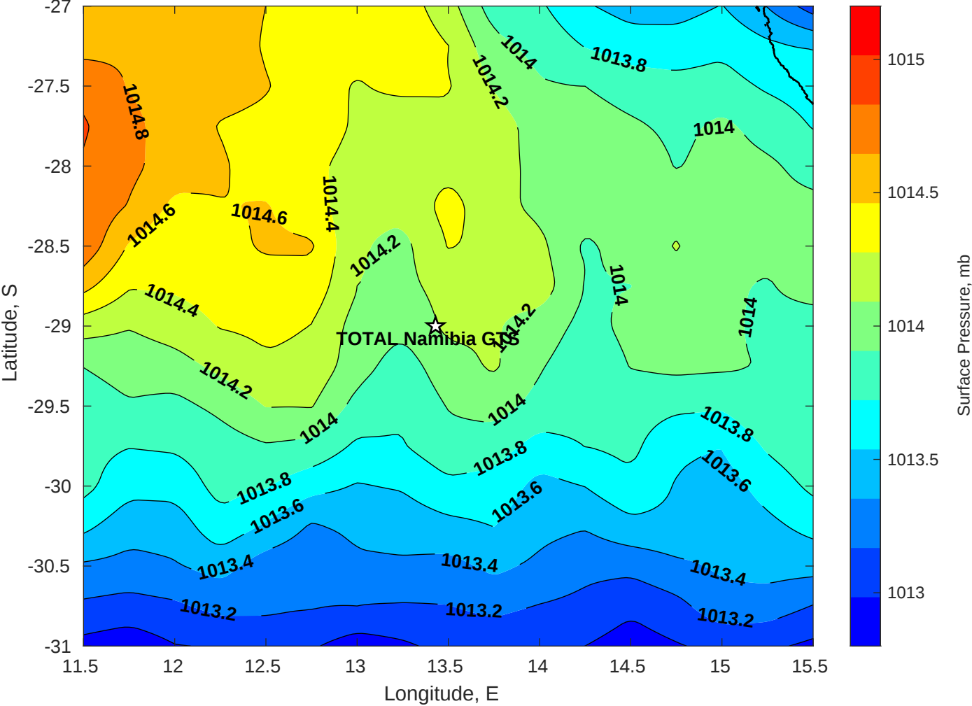
Surface Pressure (mb) for TOTAL Namibia GTS at 19-May-2025 00:00:00
