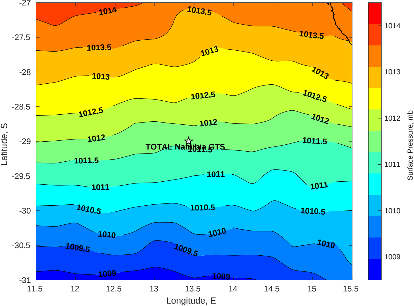
Surface Pressure (mb) for TOTAL Namibia GTS at 20-May-2025 00:00:00
