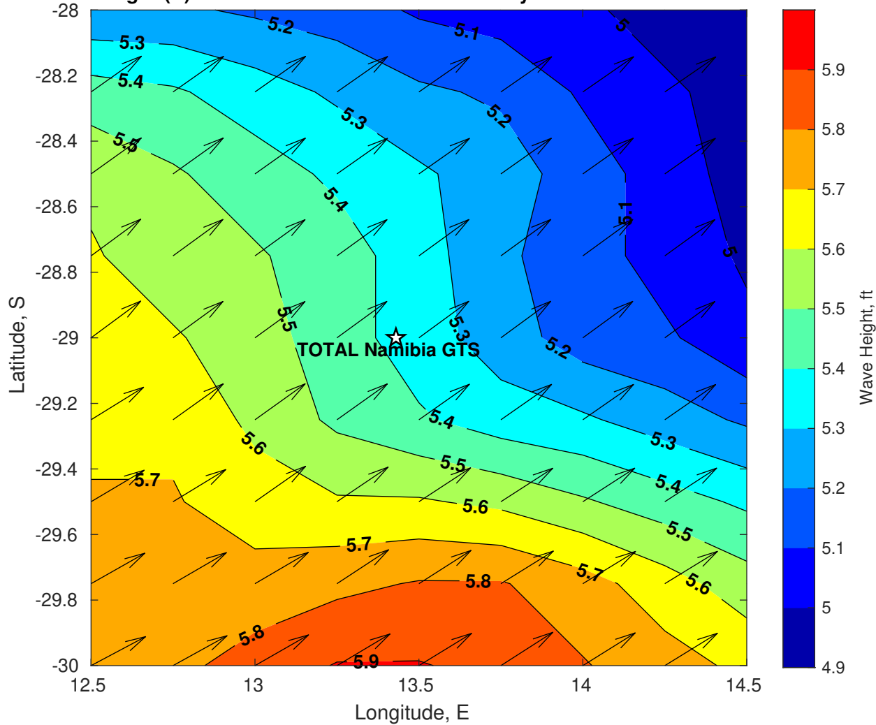
Wave Height (ft) for TOTAL Namibia GTS at 19-May-2025 09:00:00
