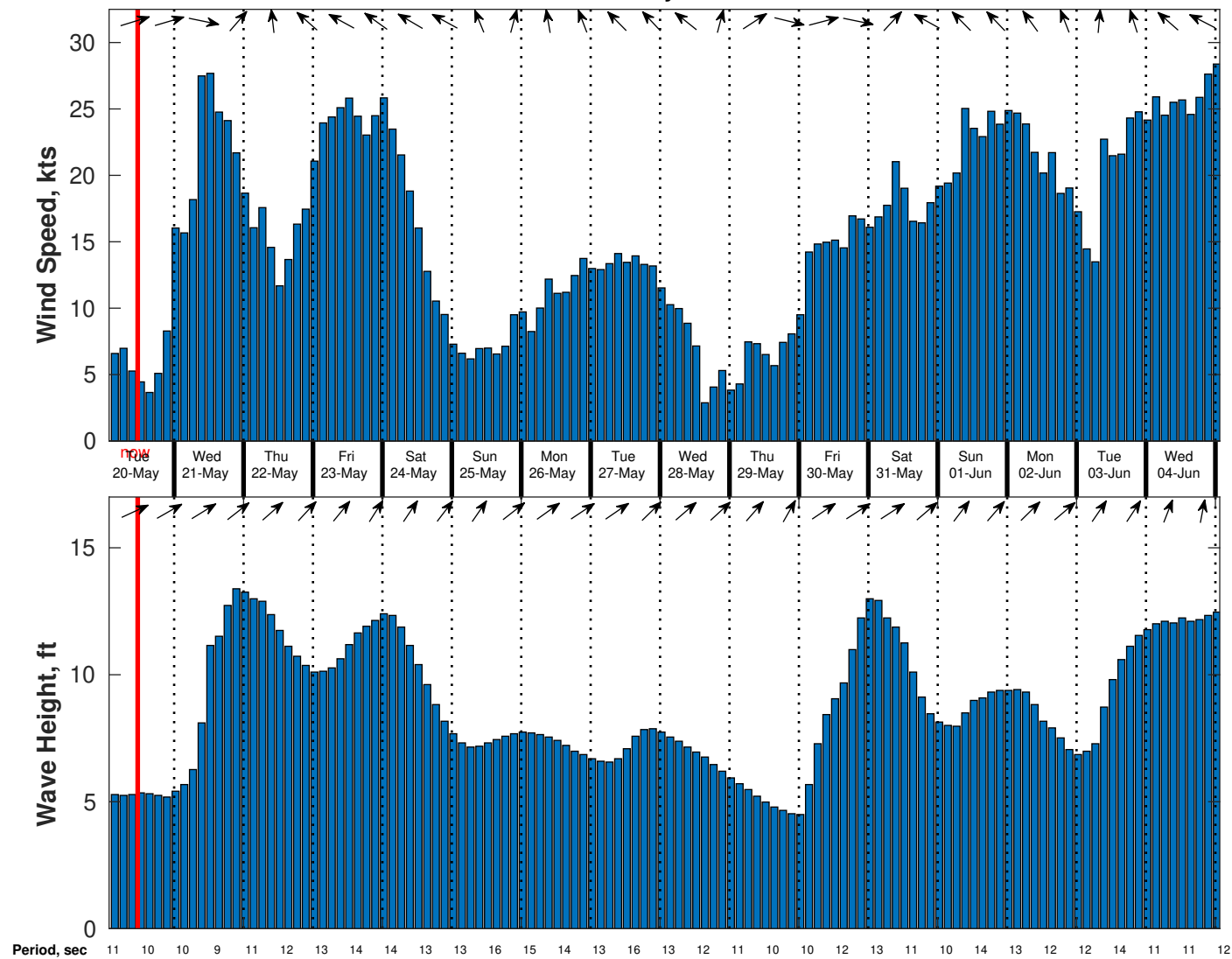
Wind & Wave Forecast for TOTAL Namibia GTS from 19-May-2025 02:00:00 to 04-Jun-2025 02:00:00
