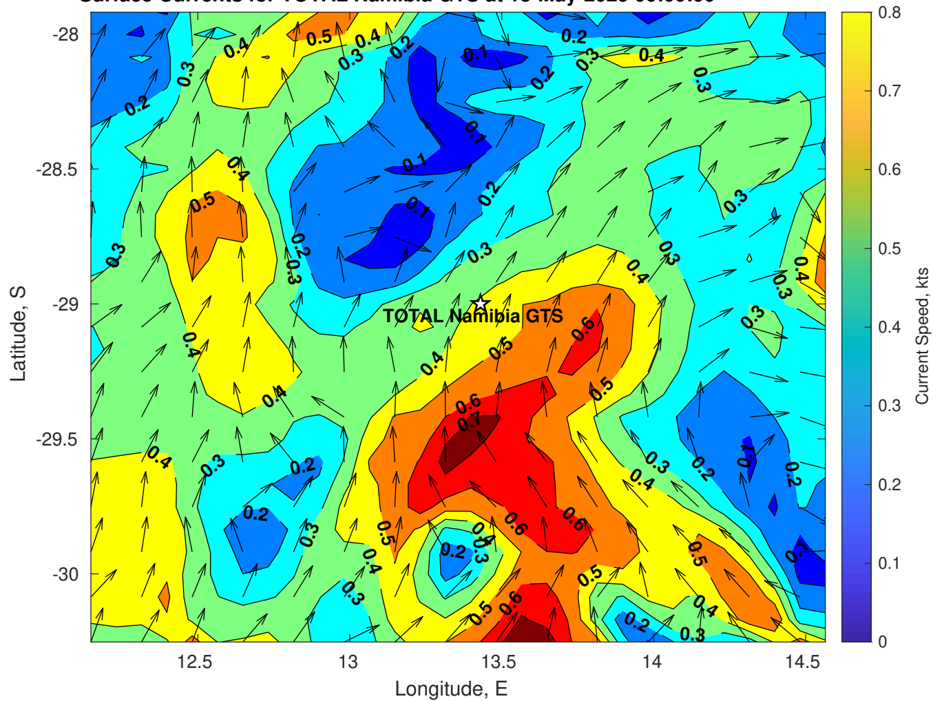
Surface Currents for TOTAL Namibia GTS at 18-May-2025 00:00:00
