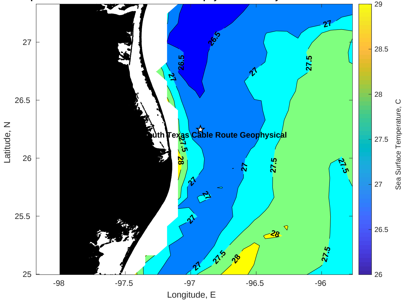
SST for Tampnet P2378 South Texas Cable Route Geophysical at 18-May-2025 00:00:00
