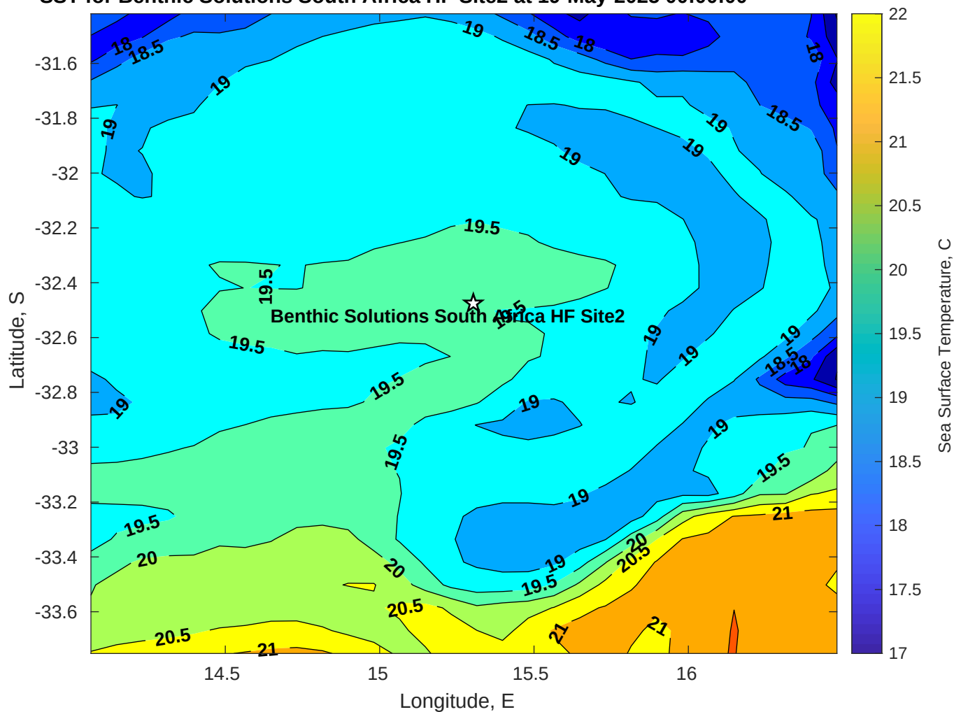
SST for Benthic Solutions South Africa HF Site2 at 19-May-2025 00:00:00
