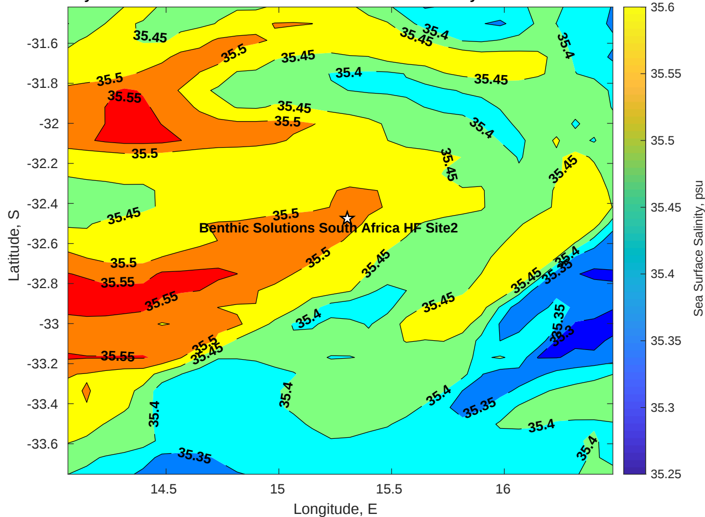
Surface Salinity for Benthic Solutions South Africa HF Site2 at 19-May-2025 00:00:00
