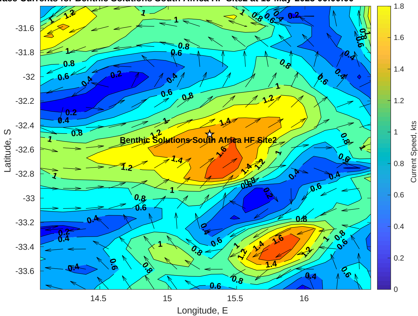
Surface Currents for Benthic Solutions South Africa HF Site2 at 19-May-2025 00:00:00
