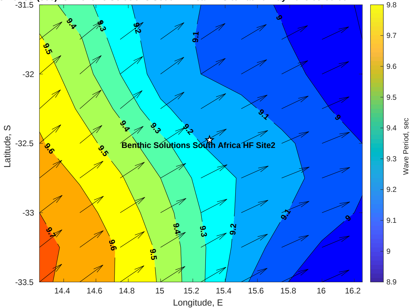
Wave Period (sec) for Benthic Solutions South Africa HF Site2 at 20-May-2025 09:00:00
