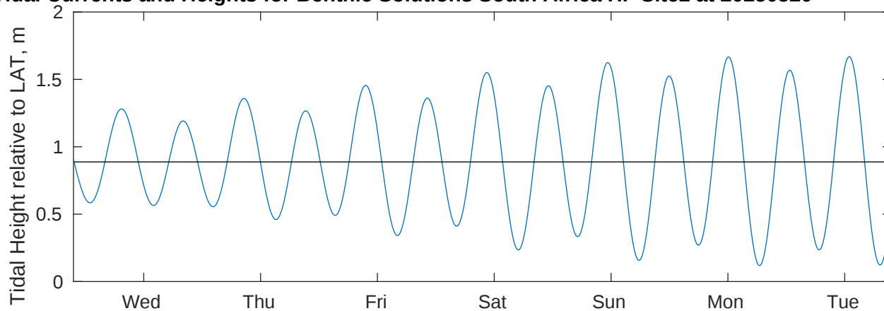
Tidal Currents and Heights for Benthic Solutions South Africa HF Site2 at 20250520
