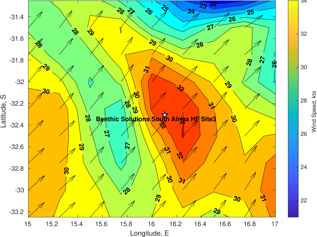
Winds (kts) for Benthic Solutions South Africa HF Site3 at 20-May-2025 09:00:00
