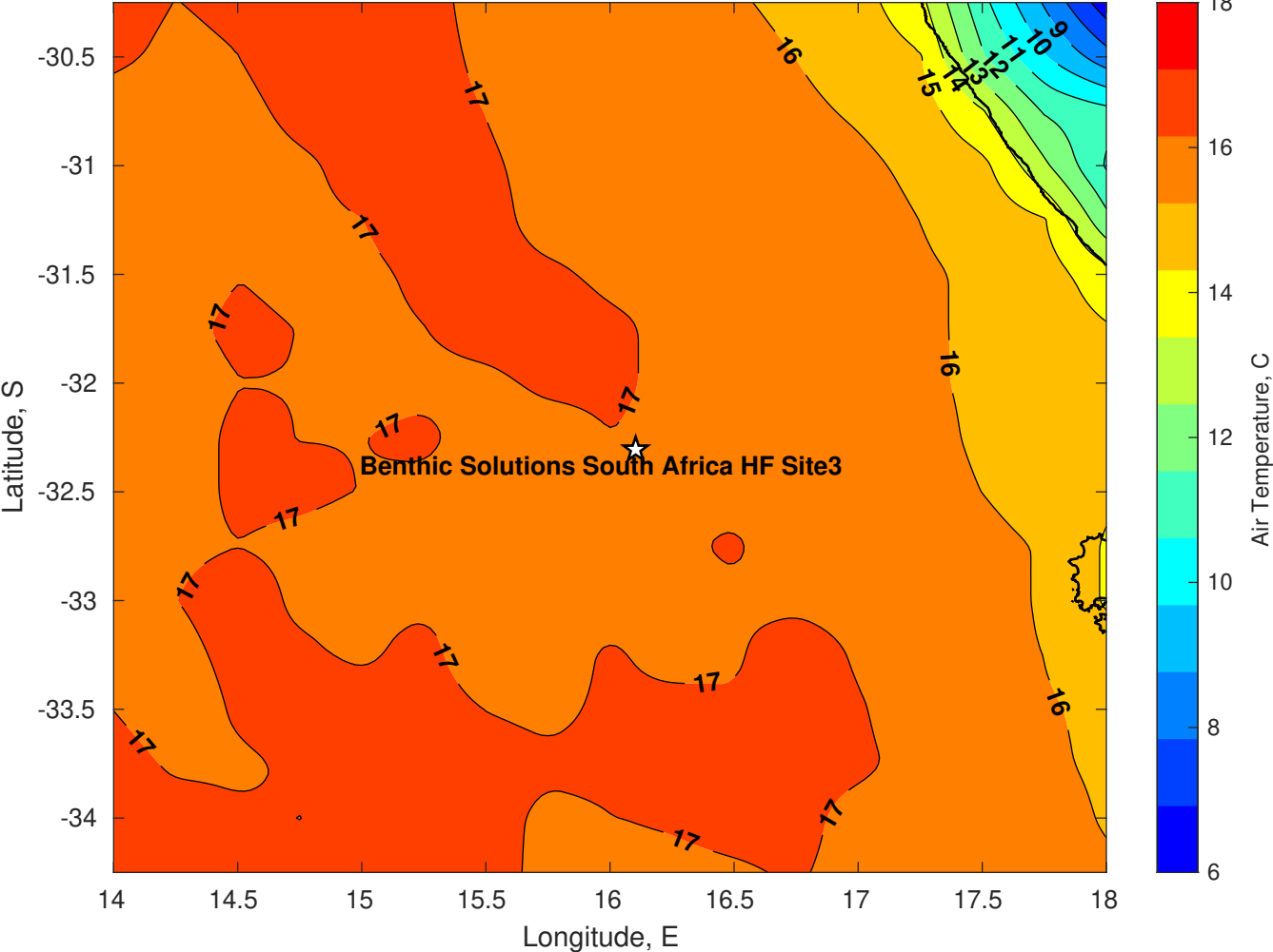
Air Temperature (C) for Benthic Solutions South Africa HF Site3 at 20-May-2025
