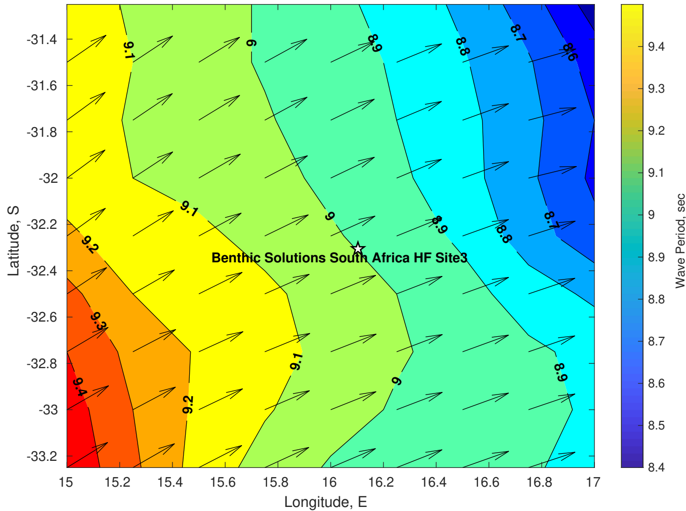
Wave Period (sec) for Benthic Solutions South Africa HF Site3 at 20-May-2025 09:00:00
