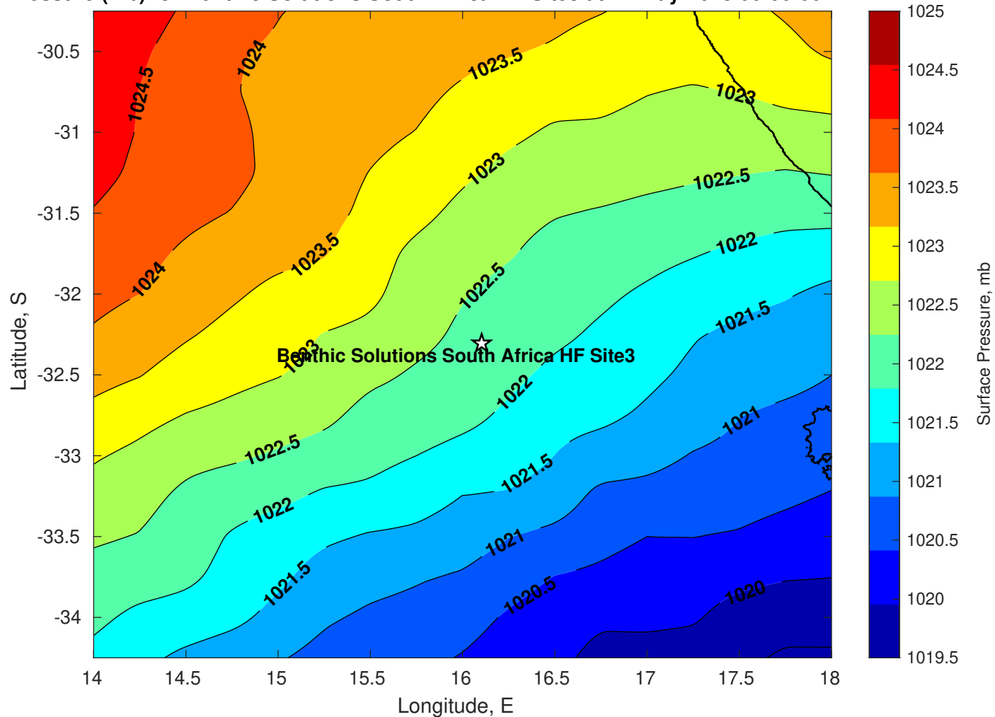
Surface Pressure (mb) for Benthic Solutions South Africa HF Site3 at 21-May-2025 00:00:00
