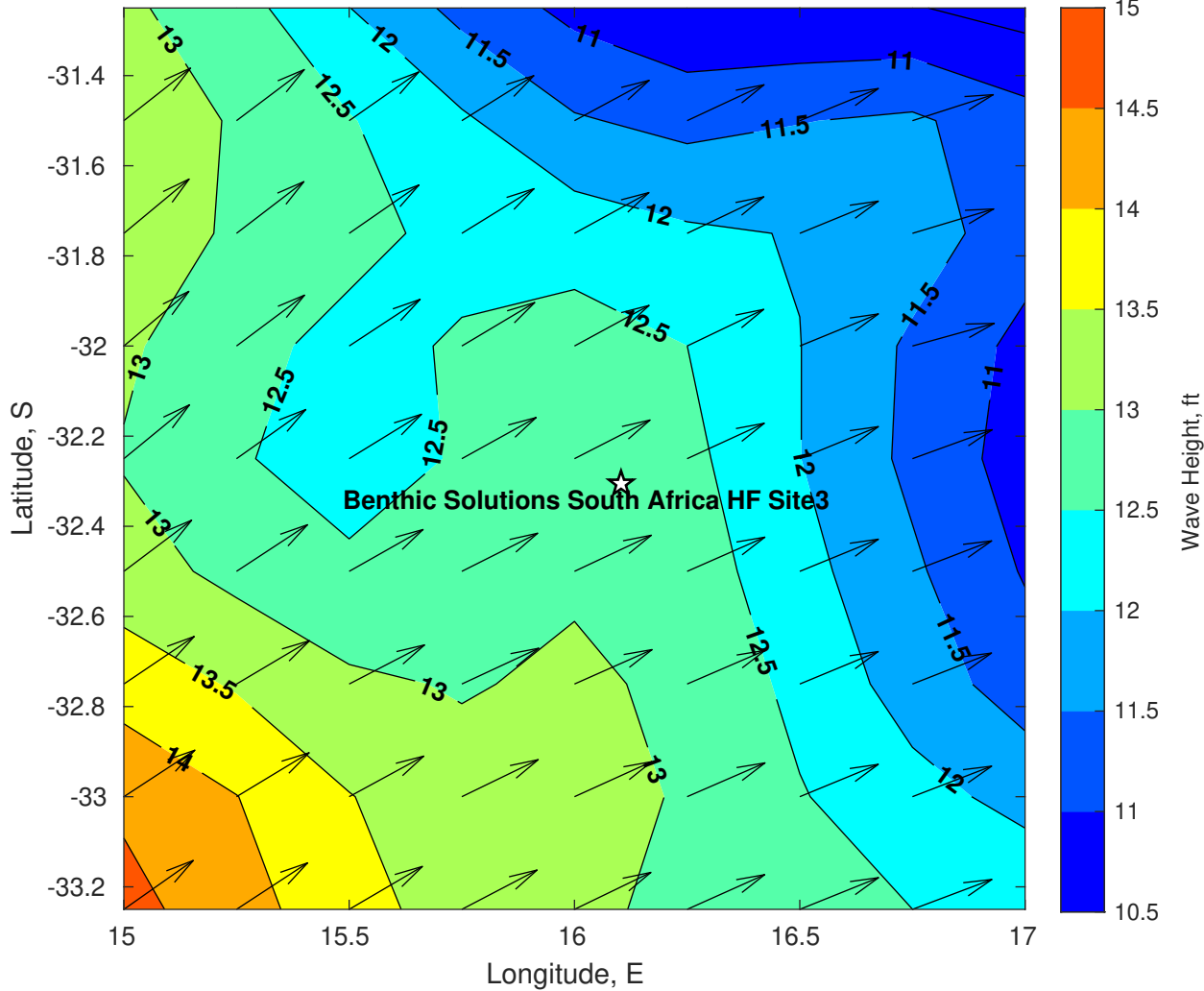
Wave Height (ft) for Benthic Solutions South Africa HF Site3 at 20-May-2025 09:00:00
