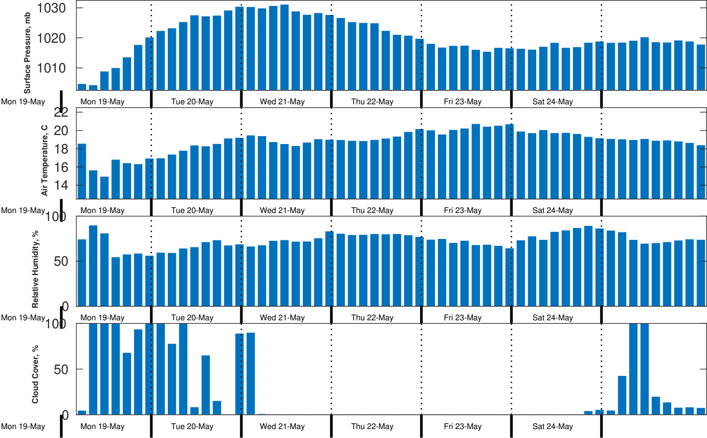
Met Forecast for Benthic Solutions South Africa HF Site3 from 20-May-2025 00:00:00 to 27-May-2025 00:00:00
