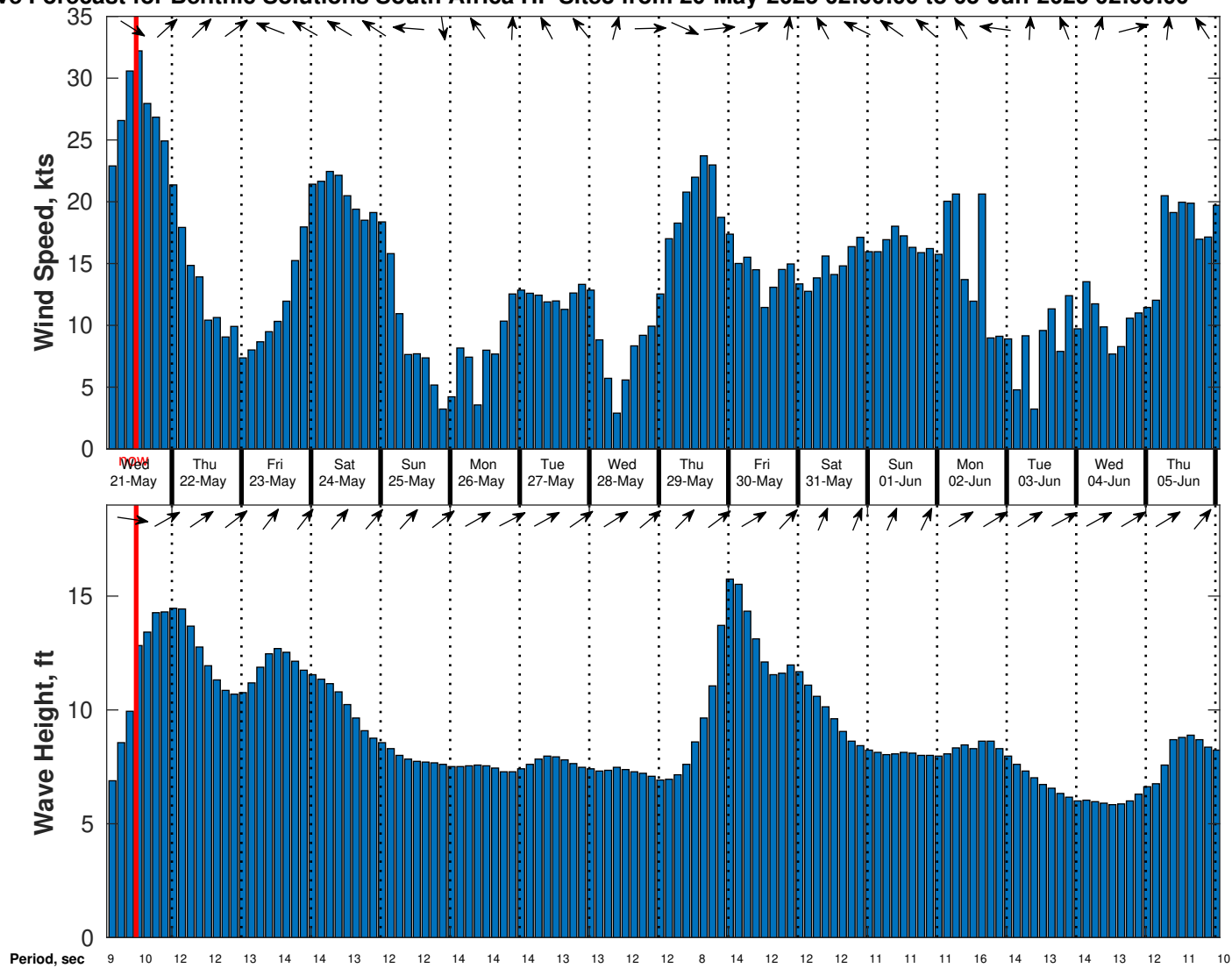
Wind & Wave Forecast for Benthic Solutions South Africa HF Site3 from 20-May-2025 02:00:00 to 05-Jun-2025 02:00:00
