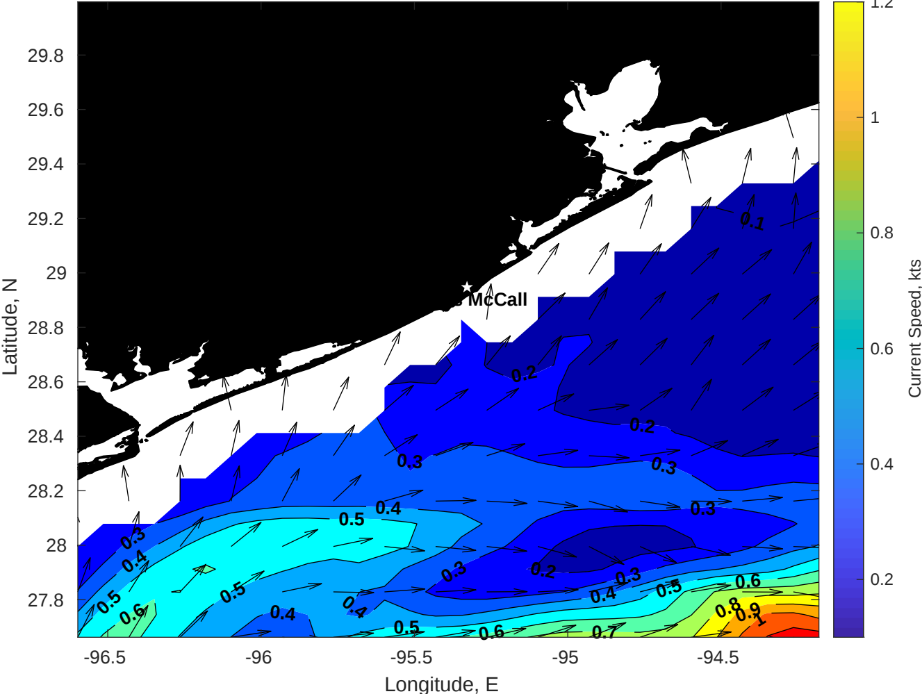
Surface Currents for Brooks McCall at 19-May-2025 00:00:00
