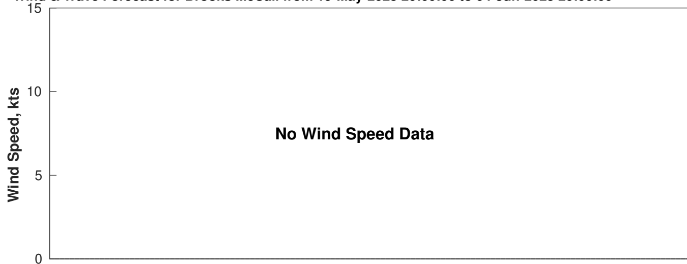
Wind & Wave Forecast for Brooks McCall from 19-May-2025 20:00:00 to 04-Jun-2025 20:00:00
