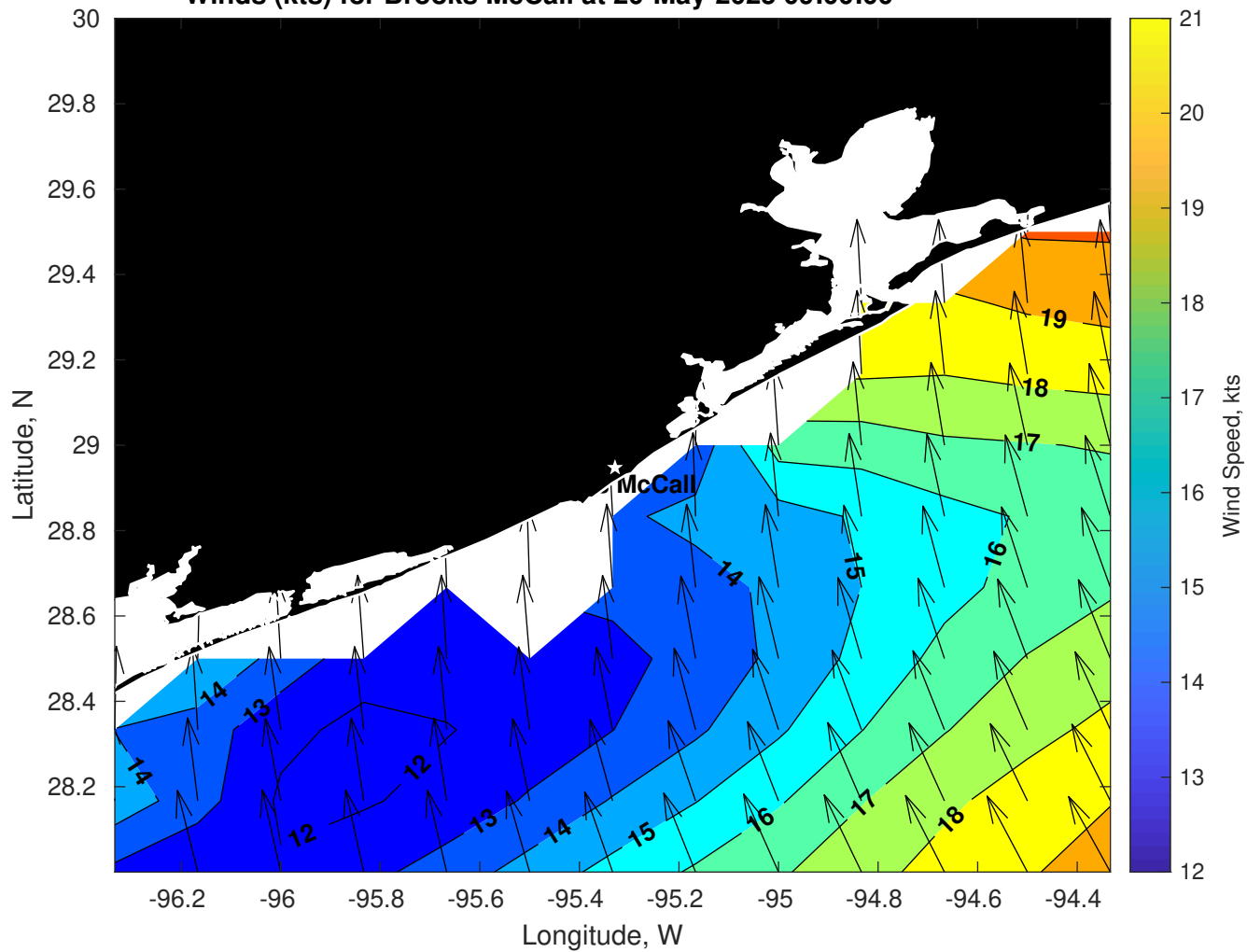
Winds (kts) for Brooks McCall at 20-May-2025 09:00:00
