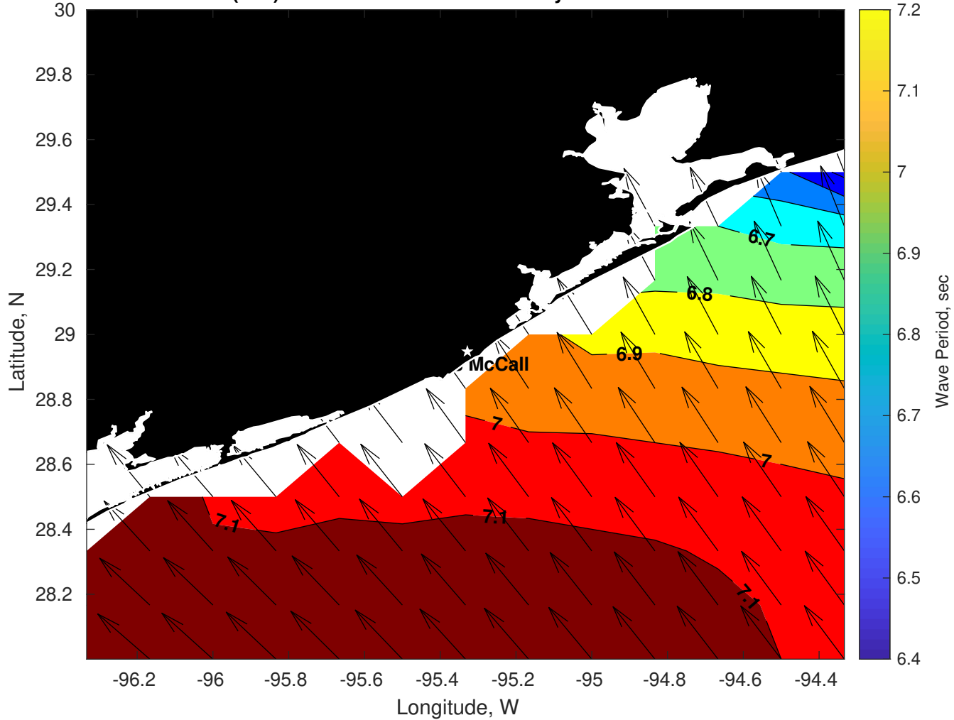
Wave Period (sec) for Brooks McCall at 20-May-2025 09:00:00
