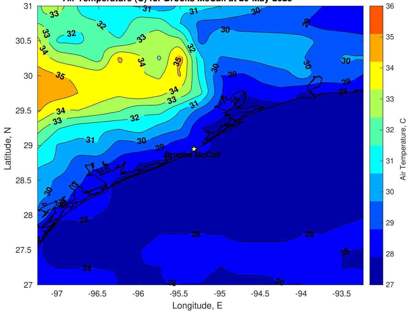
Air Temperature (C) for Brooks McCall at 20-May-2025
