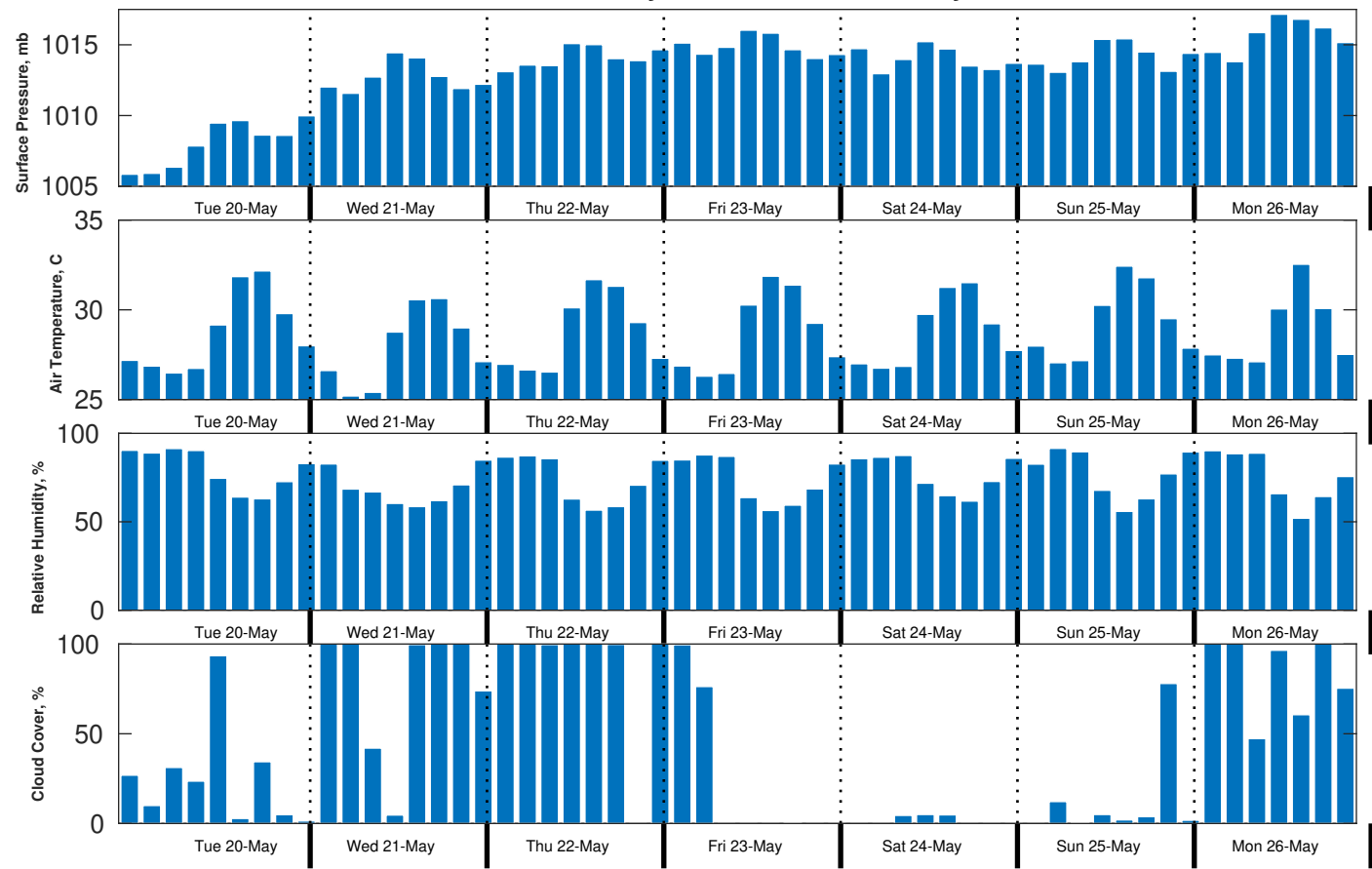
Met Forecast for Brooks McCall from 20-May-2025 00:00:00 to 27-May-2025 00:00:00
