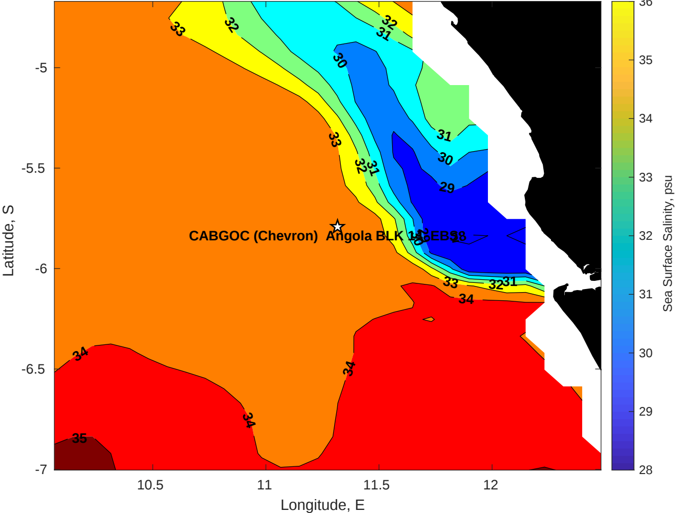
Surface Salinity for CABGOC (Chevron) Angola BLK 14 EBS at 19-May-2025 00:00:00
