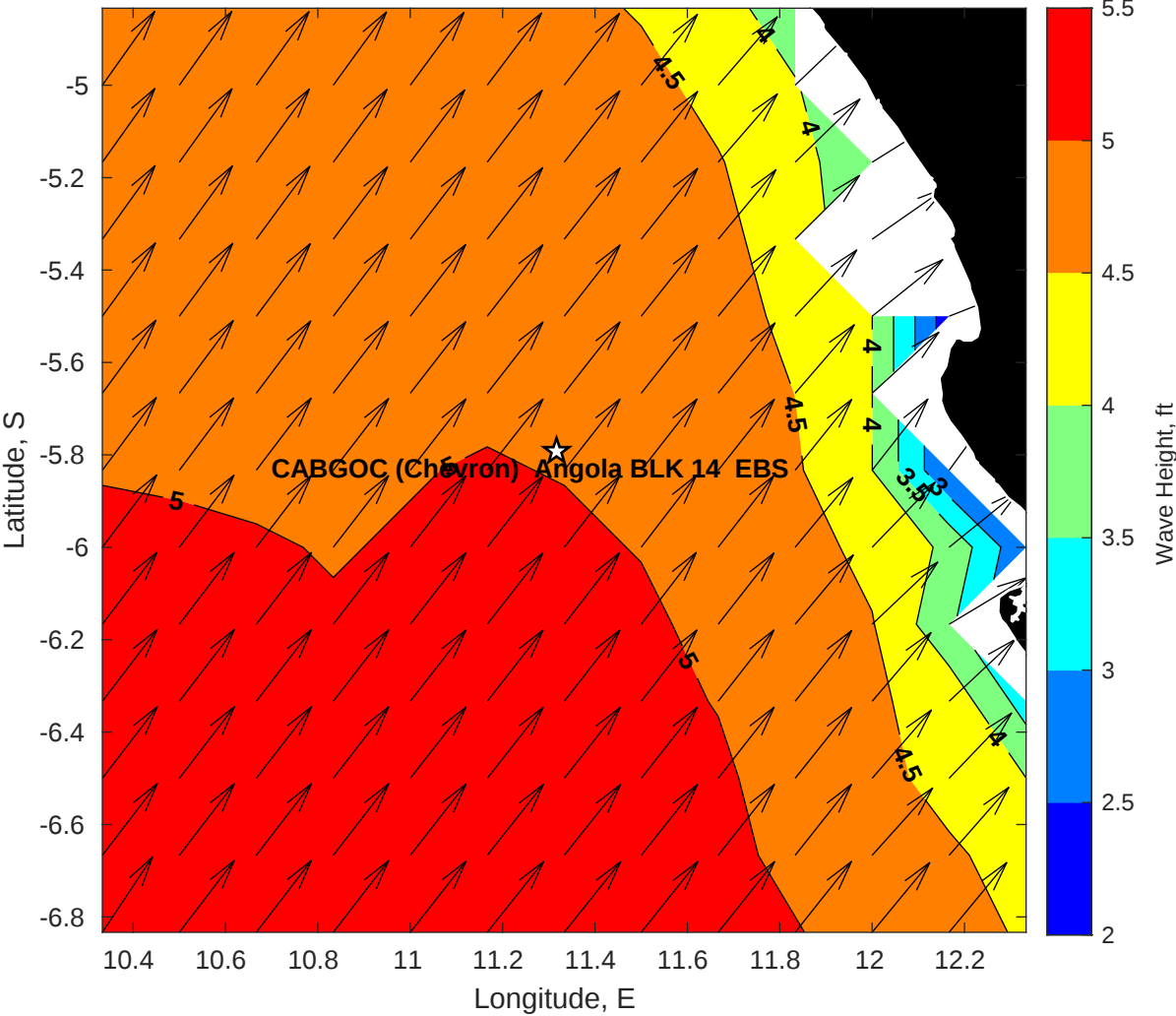
Wave Height (ft) for CABGOC (Chevron) Angola BLK 14 EBS at 20-May-2025 09:00:00
