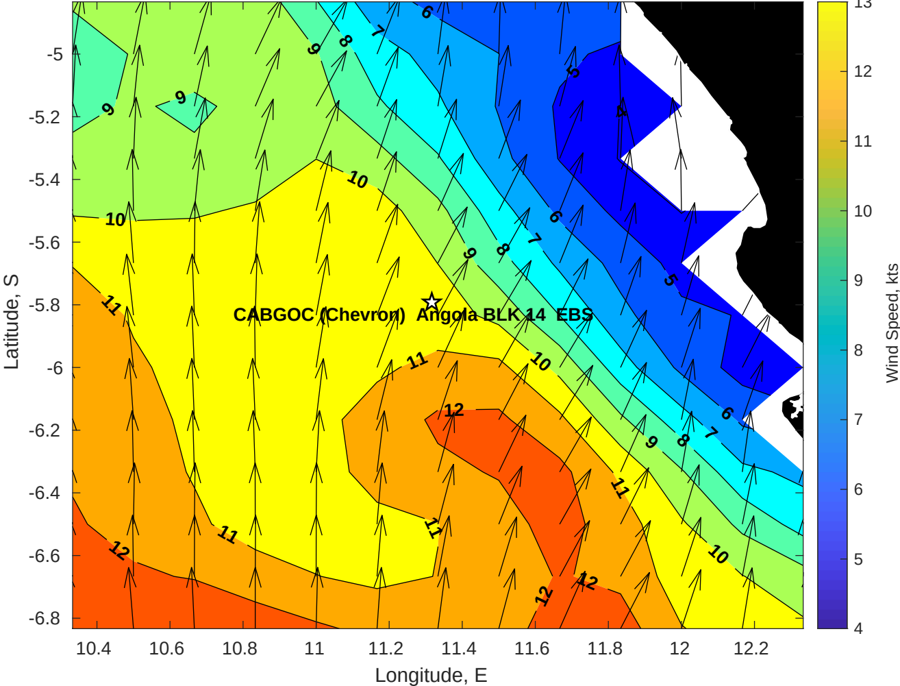
Winds (kts) for CABGOC (Chevron) Angola BLK 14 EBS at 20-May-2025 09:00:00
