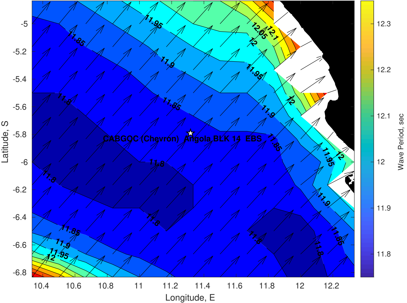
Wave Period (sec) for CABGOC (Chevron) Angola BLK 14 EBS at 20-May-2025 09:00:00
