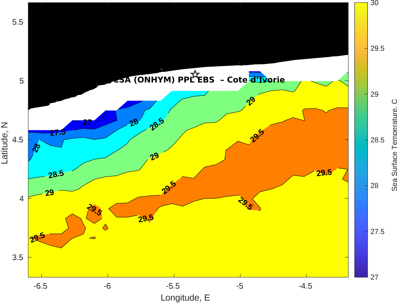
SST for CSA (ONHYM) PPL EBS - Cote d'Ivoire at 19-May-2025 00:00:00
