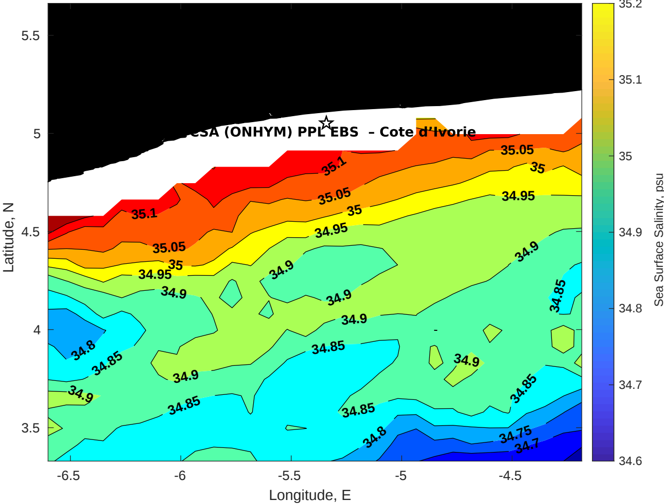
Surface Salinity for CSA (ONHYM) PPL EBS - Cote d'Ivoire at 19-May-2025 00:00:00
