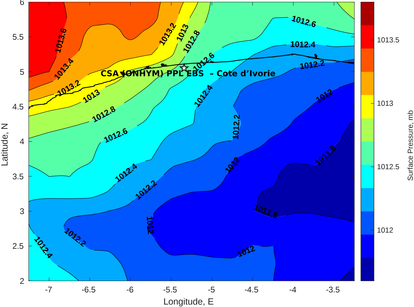
Surface Pressure (mb) for CSA (ONHYM) PPL EBS - Cote d'Ivoire at 22-May-2025 00:00:00
