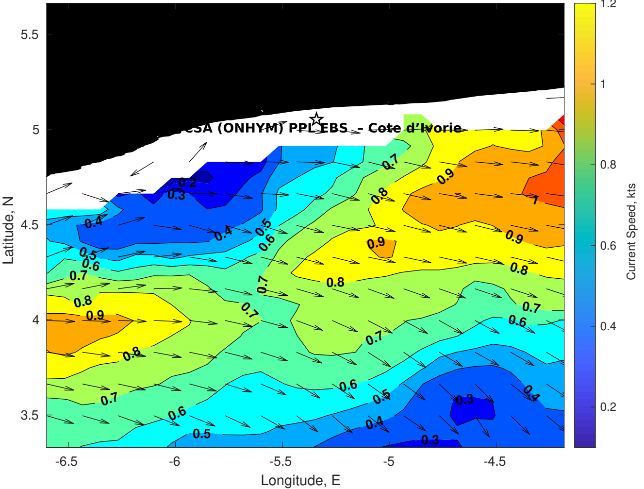
Surface Currents for CSA (ONHYM) PPL EBS - Cote d'Ivoire at 19-May-2025 00:00:00
