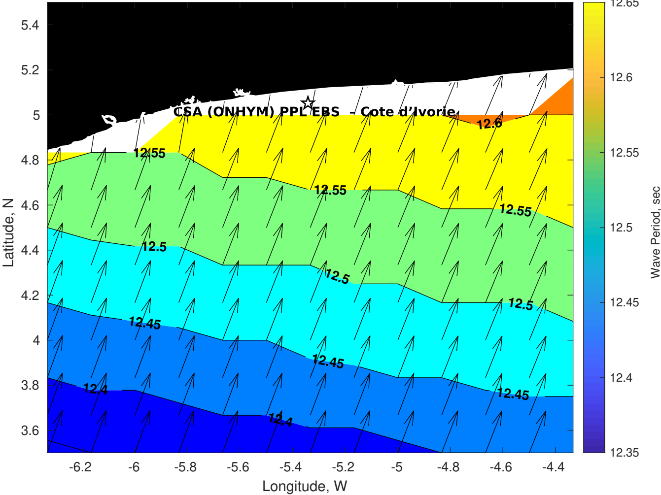
Wave Period (sec) for CSA (ONHYM) PPL EBS - Cote d'Ivoire at 20-May-2025 09:00:00
