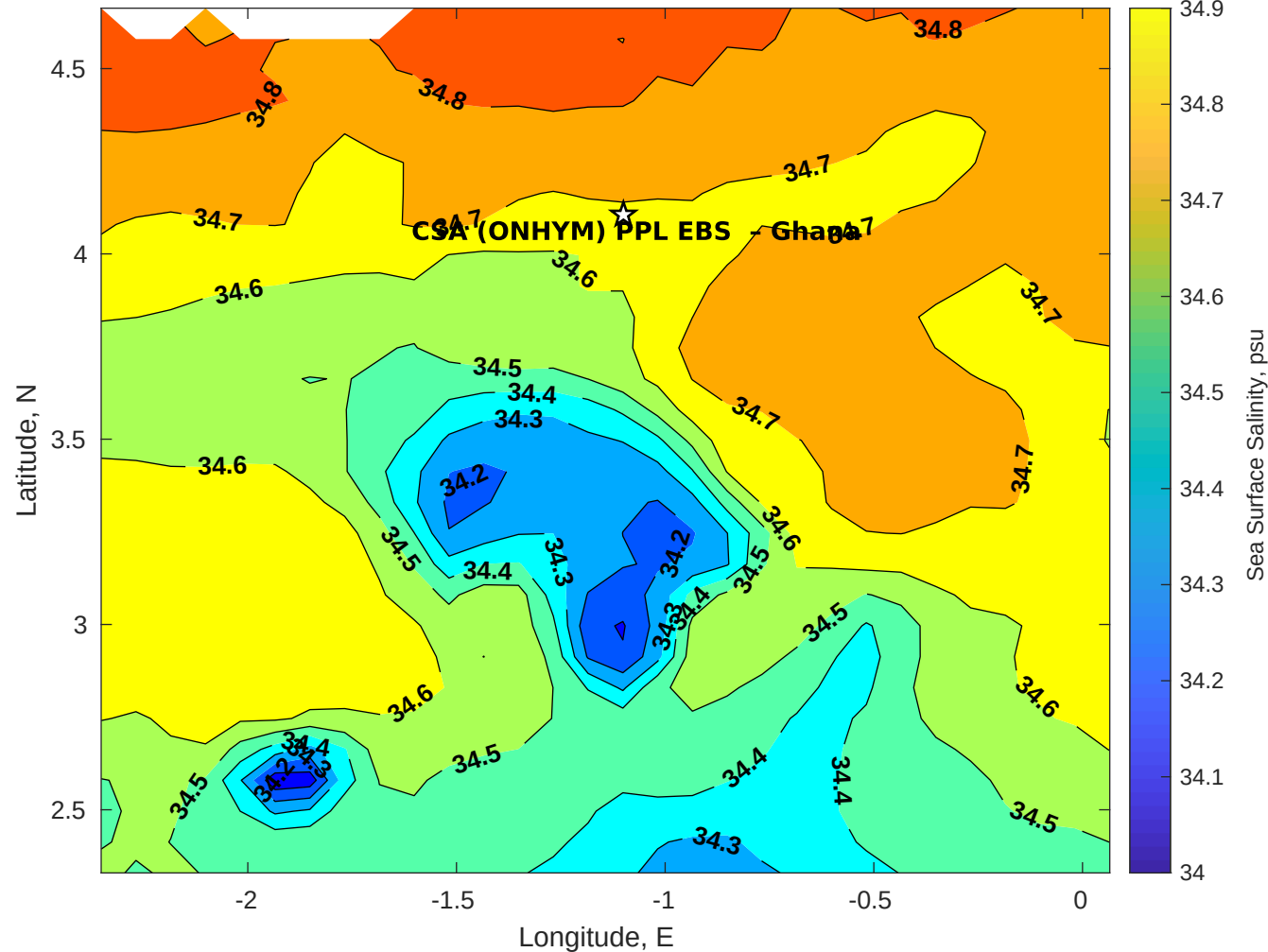
Surface Salinity for CSA (ONHYM) PPL EBS - Ghana at 19-May-2025 00:00:00
