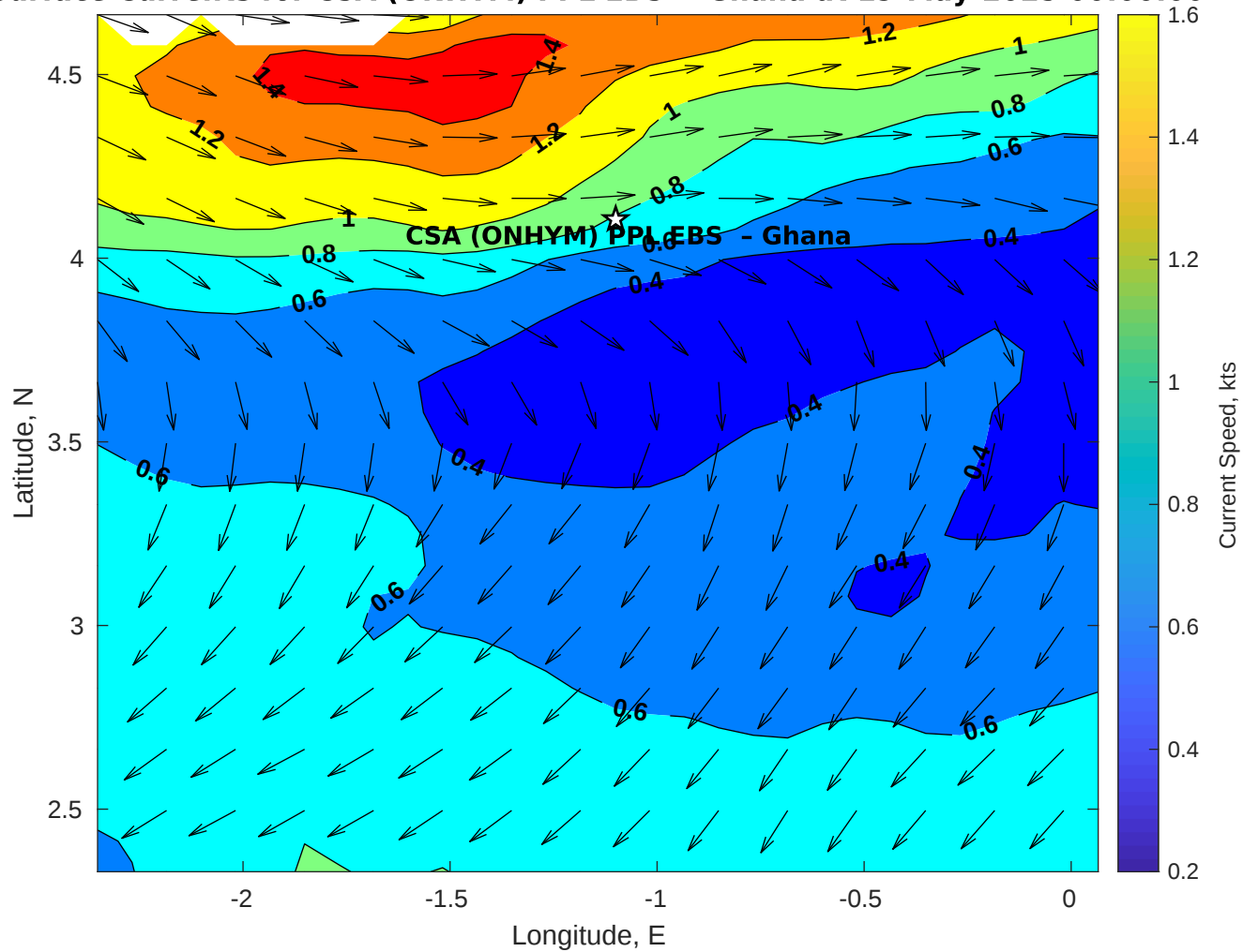
Surface Currents for CSA (ONHYM) PPL EBS - Ghana at 19-May-2025 00:00:00
