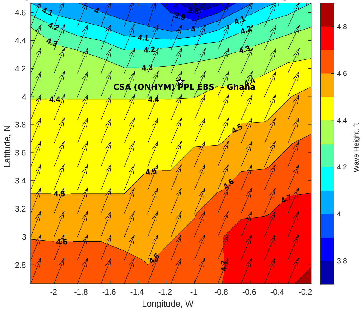
Wave Height (ft) for CSA (ONHYM) PPL EBS - Ghana at 20-May-2025 09:00:00
