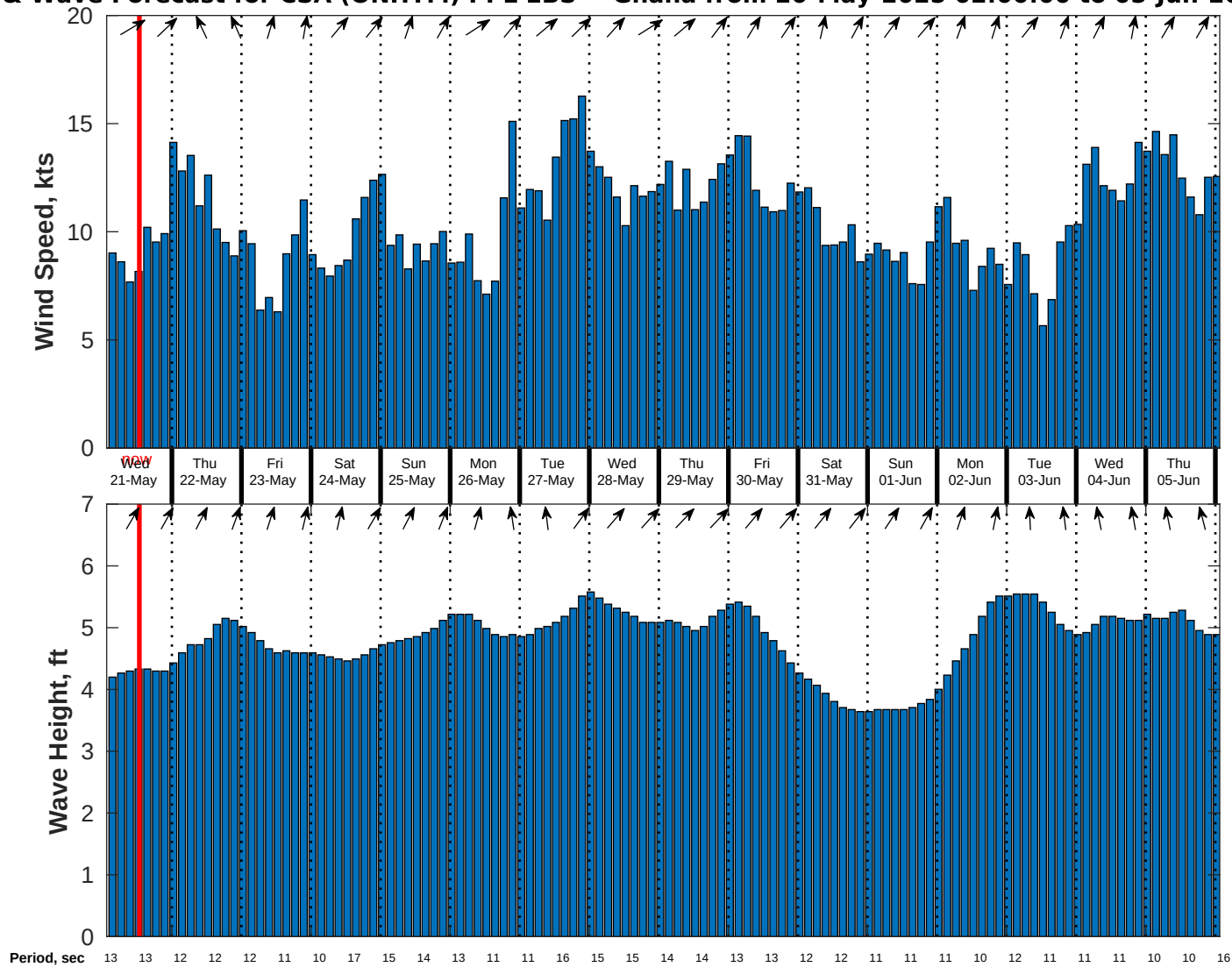
Wind & Wave Forecast for CSA (ONHYM) PPL EBS - Ghana from 20-May-2025 02:00:00 to 05-Jun-2025 02:00:00
