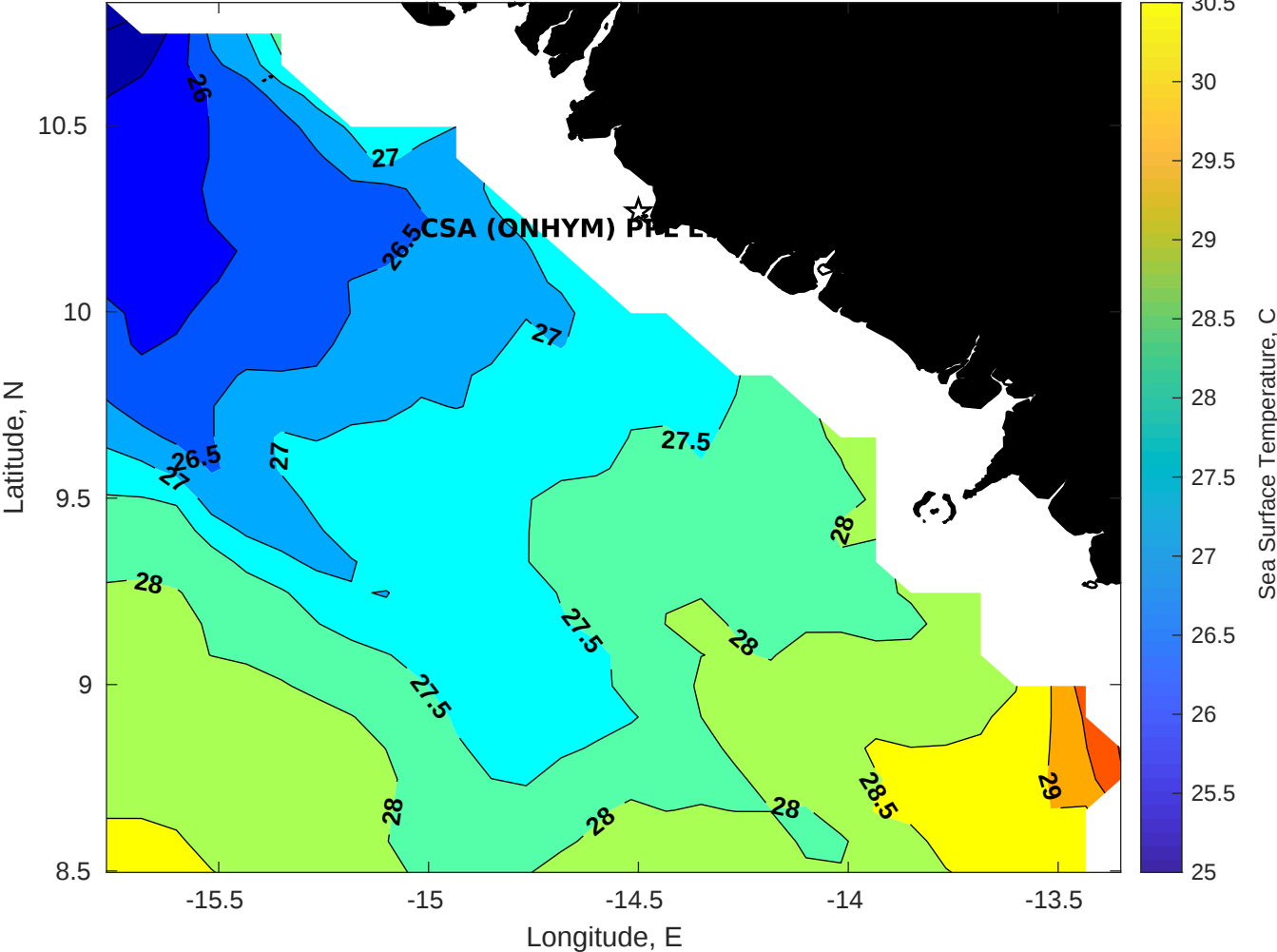
SST for CSA (ONHYM) PPL EBS - Guinea at 19-May-2025 00:00:00
