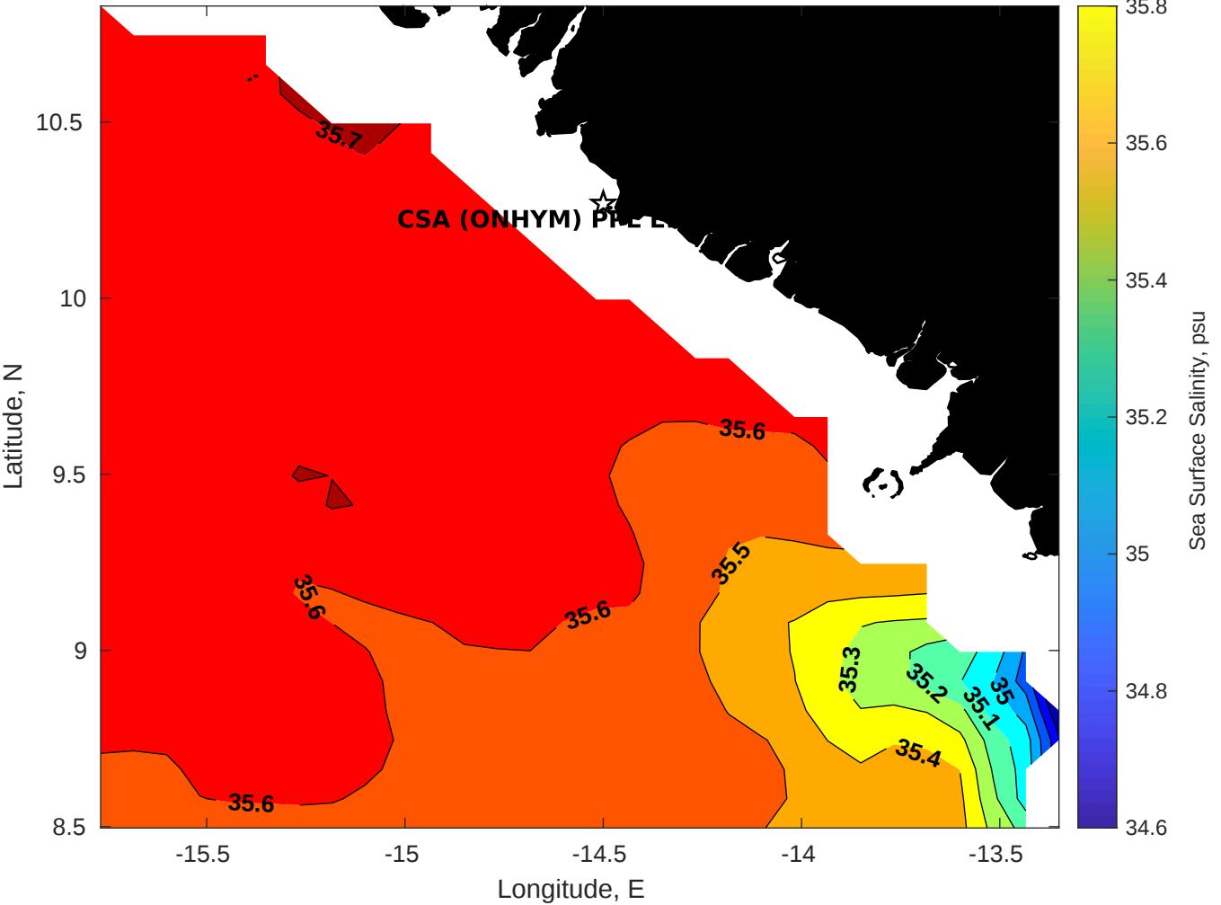
Surface Salinity for CSA (ONHYM) PPL EBS - Guinea at 19-May-2025 00:00:00
