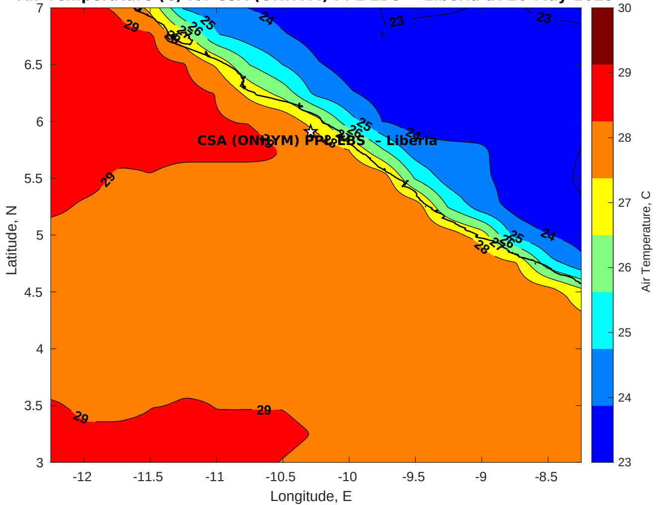
Air Temperature (C) for CSA (ONHYM) PPL EBS - Liberia at 20-May-2025
