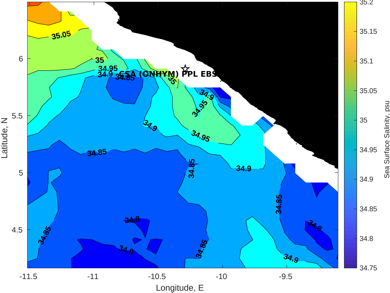
Surface Salinity for CSA (ONHYM) PPL EBS - Liberia at 19-May-2025 00:00:00
