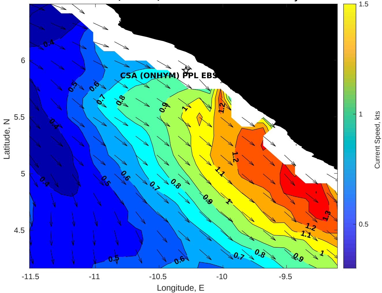
Surface Currents for CSA (ONHYM) PPL EBS - Liberia at 19-May-2025 00:00:00
