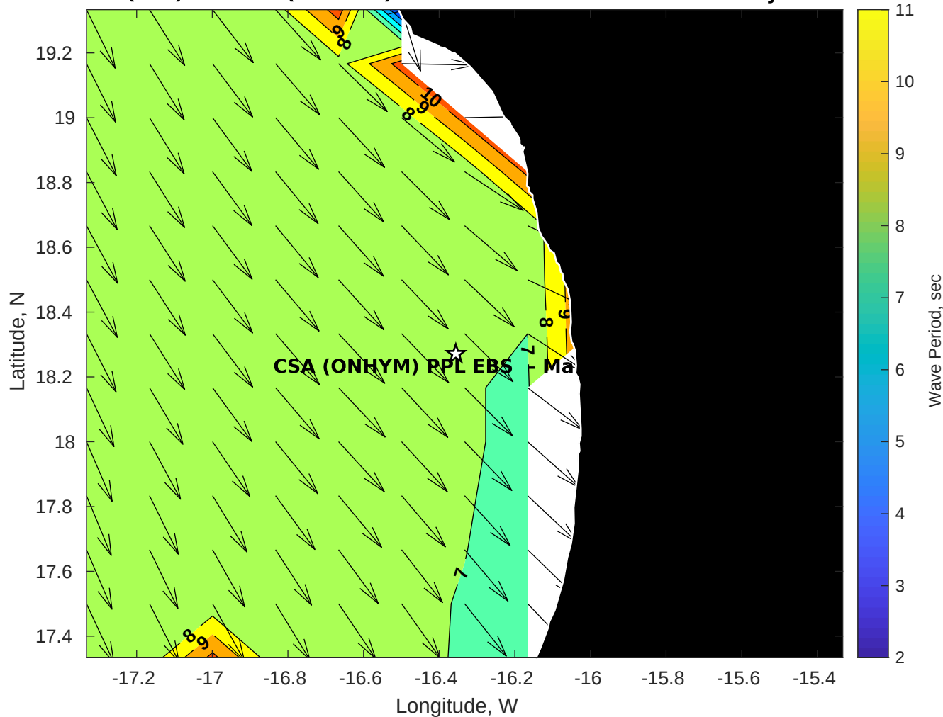
Wave Period (sec) for CSA (ONHYM) PPL EBS - Mauritania at 20-May-2025 09:00:00
