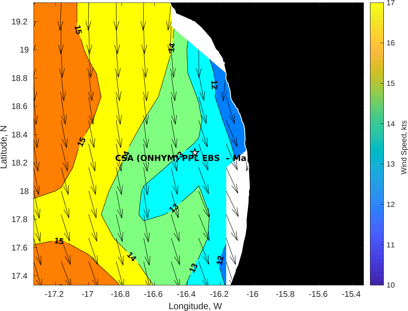
Winds (kts) for CSA (ONHYM) PPL EBS - Mauritania at 20-May-2025 09:00:00
