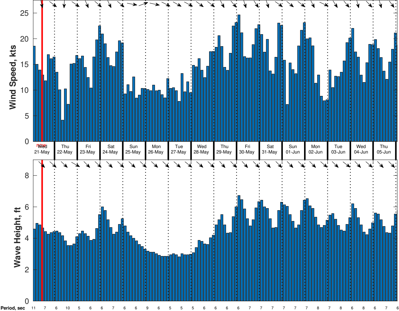
Wind & Wave Forecast for CSA (ONHYM) PPL EBS - Mauritania from 20-May-2025 01:00:00 to 05-Jun-2025 01:00:00
