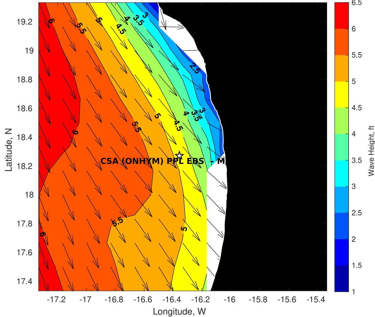
Wave Height (ft) for CSA (ONHYM) PPL EBS - Mauritania at 20-May-2025 09:00:00
