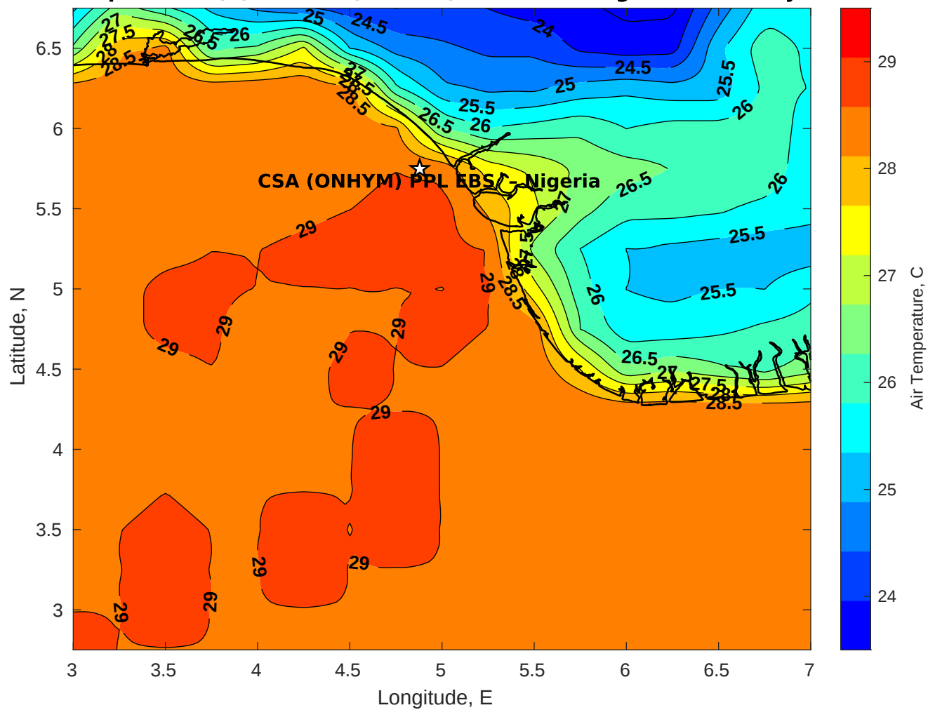
Air Temperature (C) for CSA (ONHYM) PPL EBS - Nigeria at 20-May-2025
